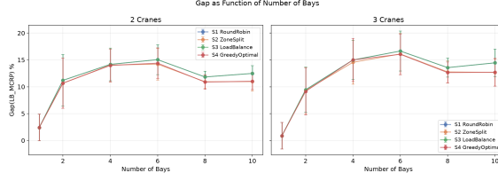
Figure A.4: \text{Gap}(\text{LB}_{\text{MCRP}})\% as a function of the number of bays, for each strategy at C=2 (left) and C=3 (right).
