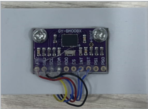
BNO085 breakout (GY-BNO08X), I²C to MCU
