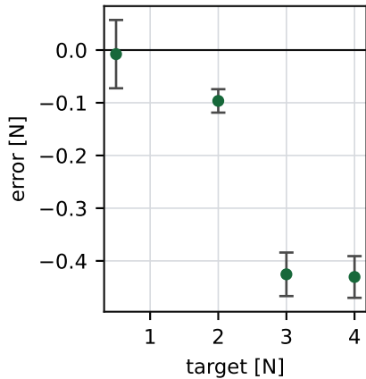
Steady-state error (mean \pm SD)
