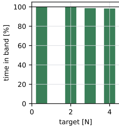
Time inside the deadband
