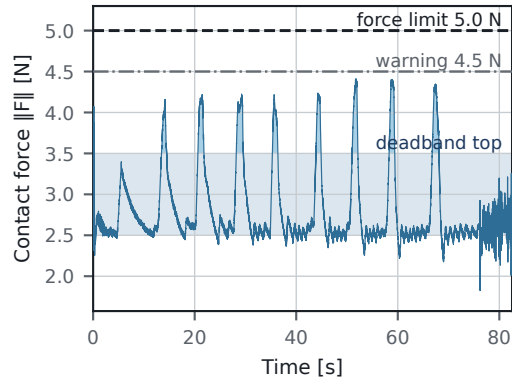
(b) Repeated rapid injections at the 3.0 N setpoint
