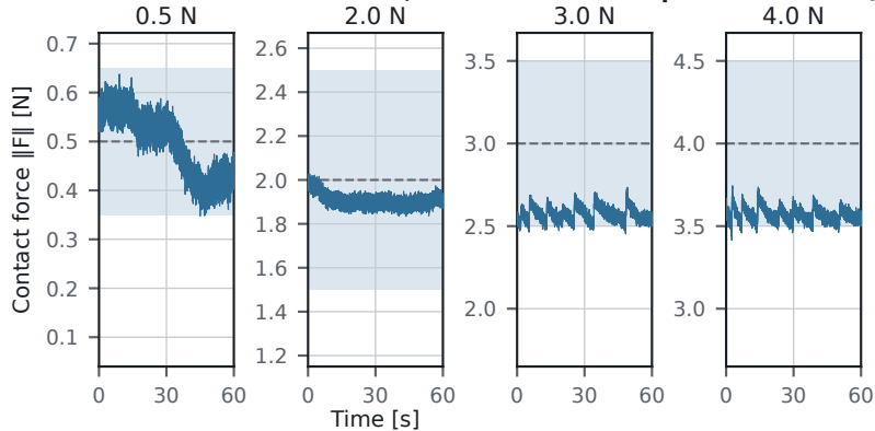
(a) 60 s holds — shaded band is the deadband, dashed line the setpoint
