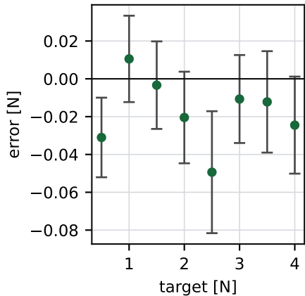
Steady-state error (mean \pm SD)
