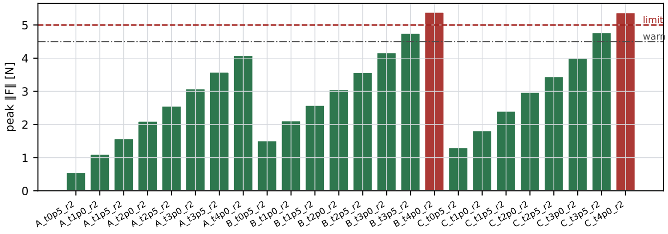
Worst force seen in each run, against the configured limits
