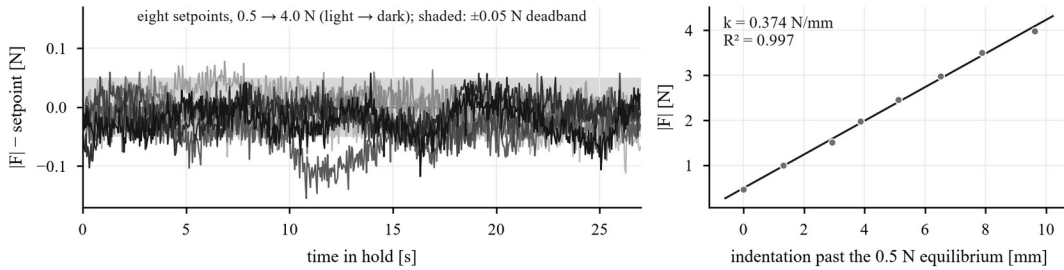
Force hold at eight set points. Left: error from the commanded force during the scored part of each hold, all eight set points from 0.5–4.0 N overlaid (light to dark), with the \pm 0.05 N dead band shaded; the first 3 s of each hold are discarded and the traces are 1 kHz samples pooled over two independently calibrated sessions. Right: the equilibrium force against indentation past the 0.5 N point, whose slope is the phantom stiffness used in the time constant above.
