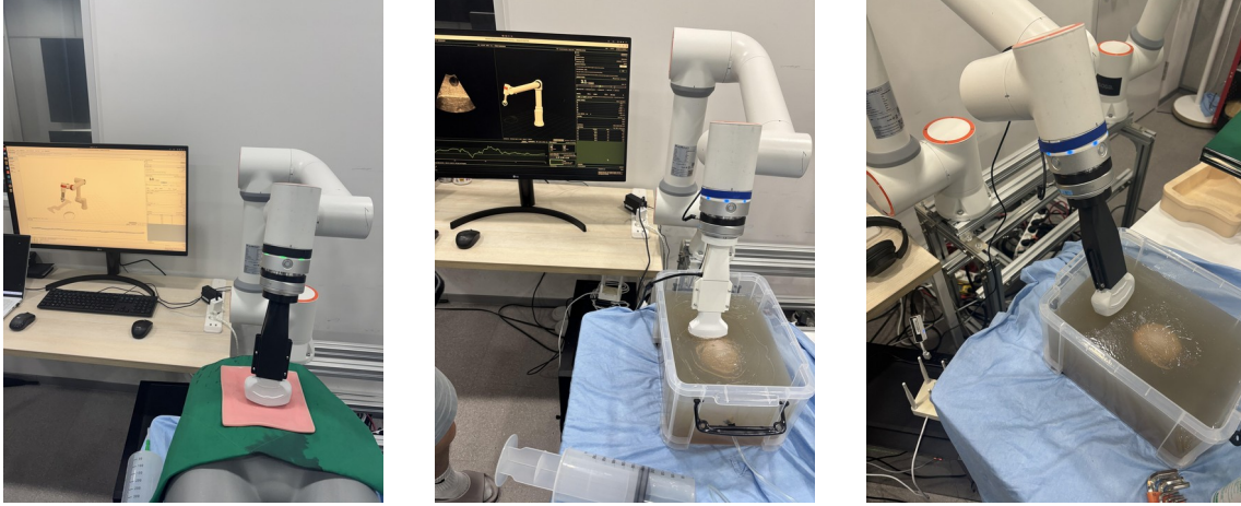
The three benches. (a) Force experiments: an inflatable air tube inside a torso mannequin, inflated and deflated through a 500 mL syringe while the robot holds a commanded force. (b) Final setup: the clinical probe on the gel bladder phantom in its water bath, with the syringe line that fills and empties the lumen and the console the operator watches. (c) Contact stiffness: a printed probe replica indents the gel while force comes from the force/torque sensor and depth from forward kinematics, so neither the scanner nor the control stack is involved (force noise 0.015 N, depth noise 0.4 \mu\text{m} , indentation steps about 1 mm).
