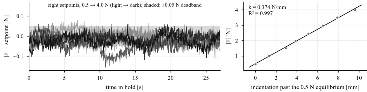
Force hold at eight set points. Left: error from the commanded force during the scored part of each hold, all eight set points from 0.5–4.0 N overlaid (light to dark), with the \pm 0.05 N dead band shaded; the first 3 s of each hold are discarded and the traces are 1 kHz samples pooled over two independently calibrated sessions. Right: the equilibrium force against indentation past the 0.5 N point, whose slope is the phantom stiffness used in the time constant above.
