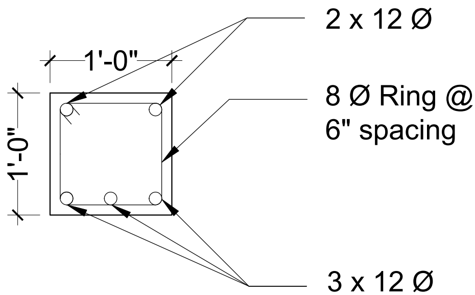
Tie Beam Detail
