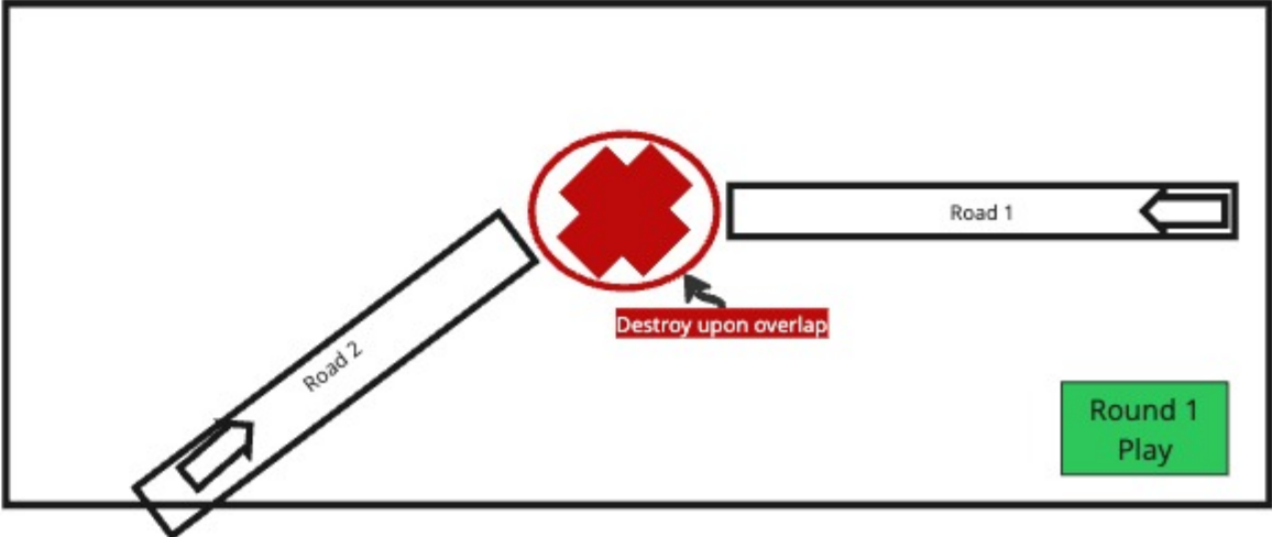
Map Mockup
