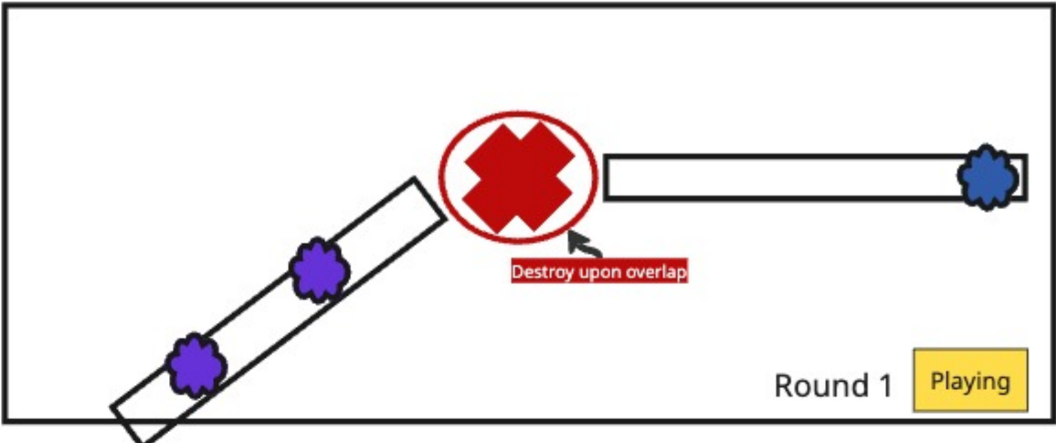
Round Mockup
