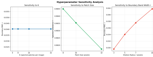
Fig. 4. Sensitivity of B-MAE and S-Coh to (left) number of patches per image k , (centre) patch size p_s , and (right) boundary dilation radius d . B-MAE is stable across k ; smaller patches improve S-Coh; smaller dilation improves B-MAE.
