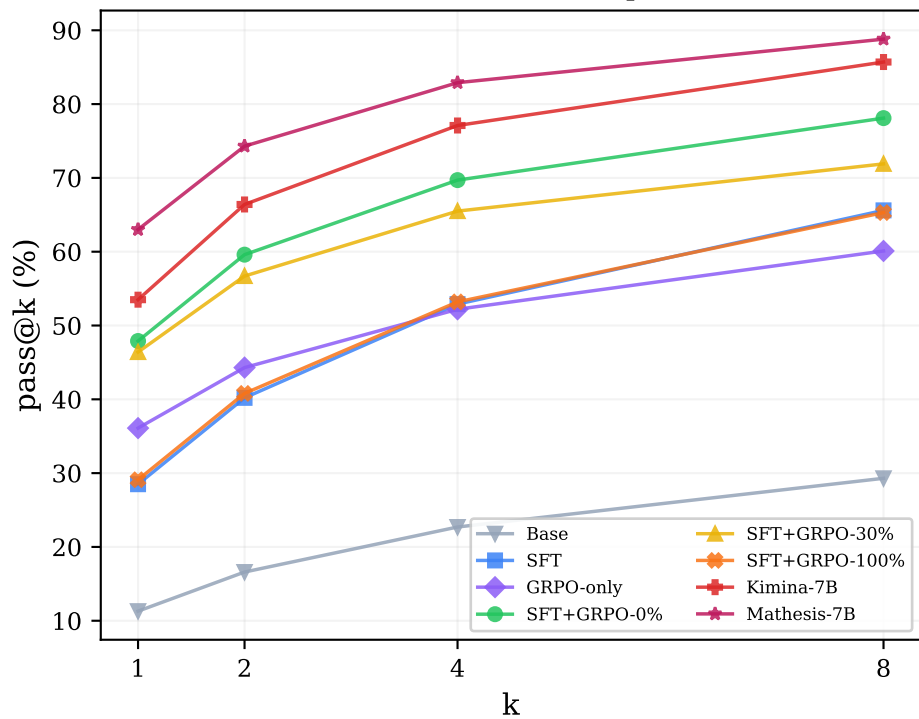
PutnamBench (Compile)
