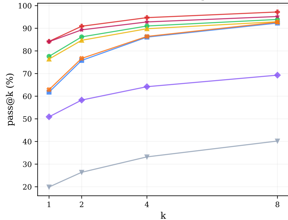
Gaokao-Formal (Compile)
