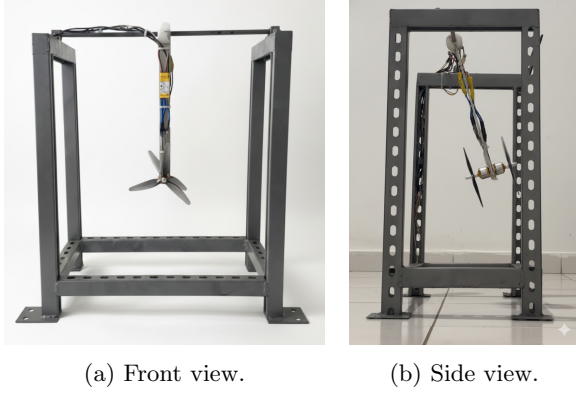
Fig. 2: The developed twin-rotor aeropendulum experimental platform from front and side perspectives.
