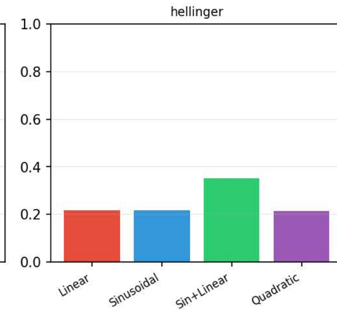
Joint vs Pointwise — Prior: low_noise — \tau \approx 1.0
