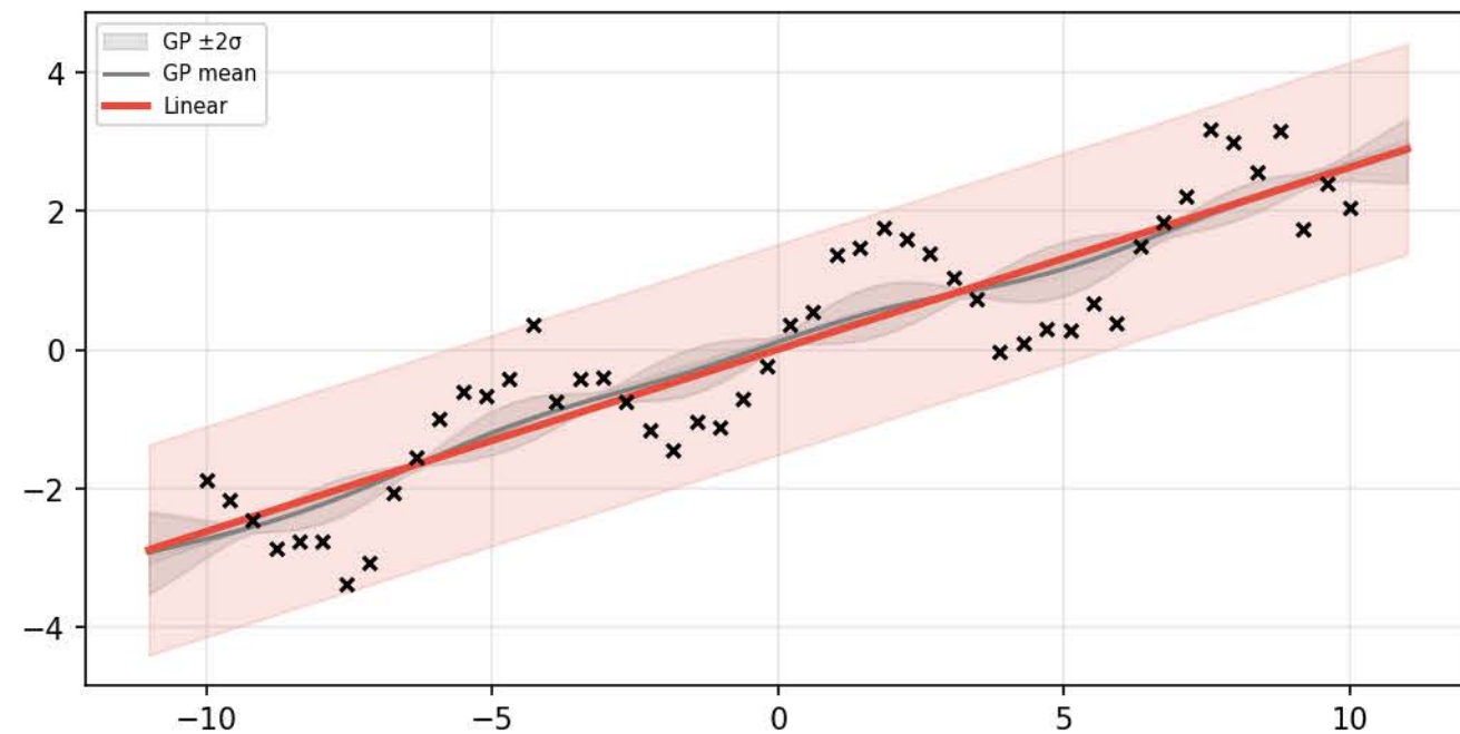
Sin+Linear
