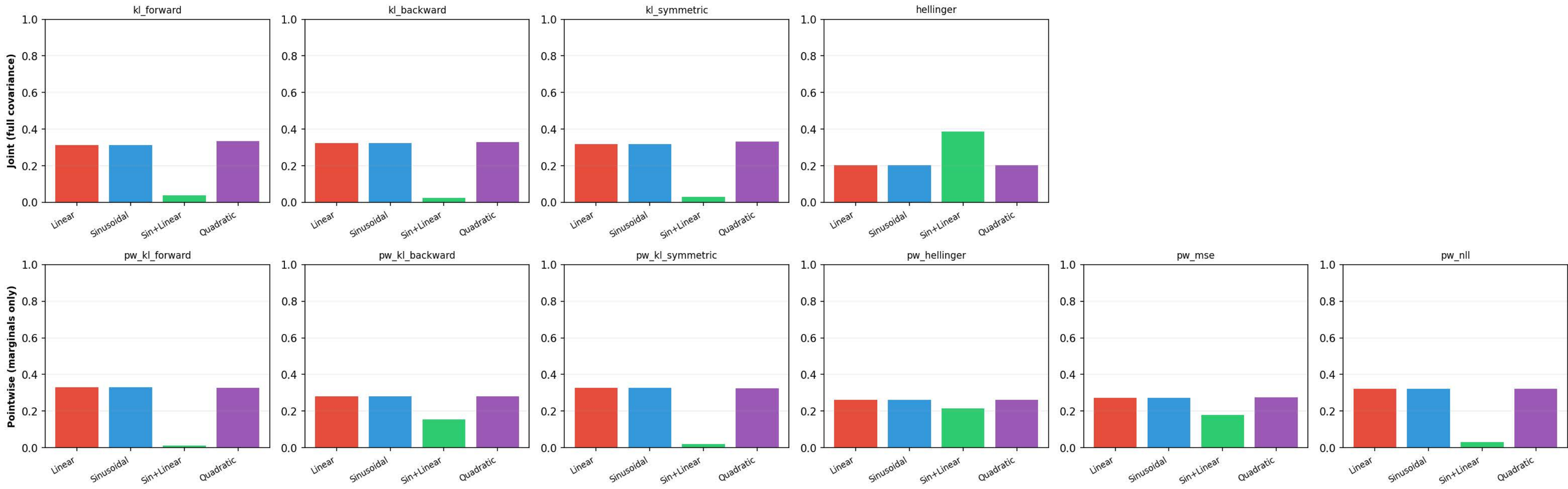
Joint vs Pointwise — Prior: informative — \tau \approx 1.0
