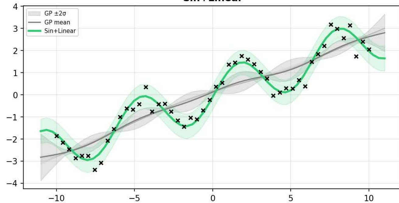
Sin+Linear
