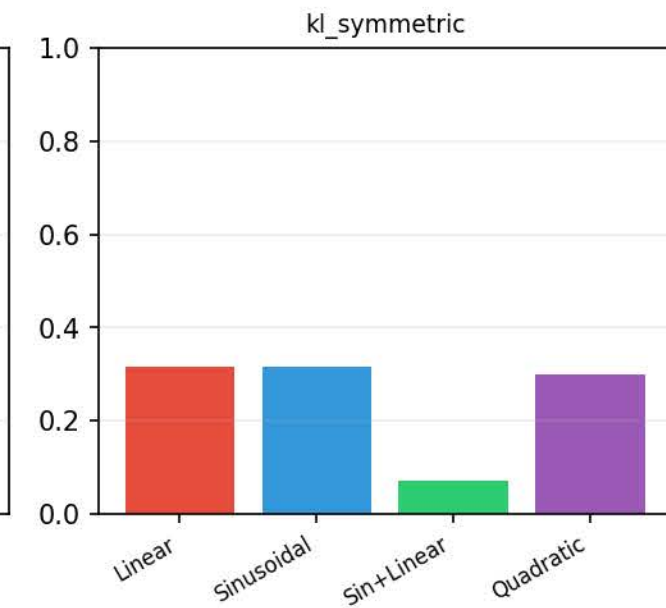
Joint vs Pointwise — Prior: high_noise — \tau \approx 1.0
