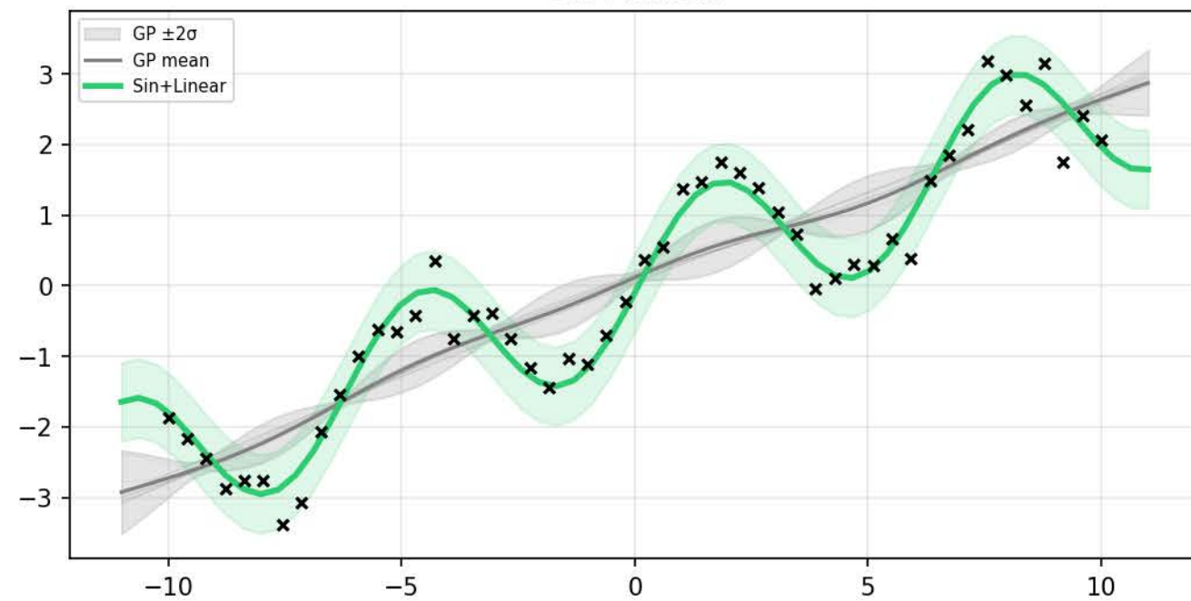
Sin+Linear
