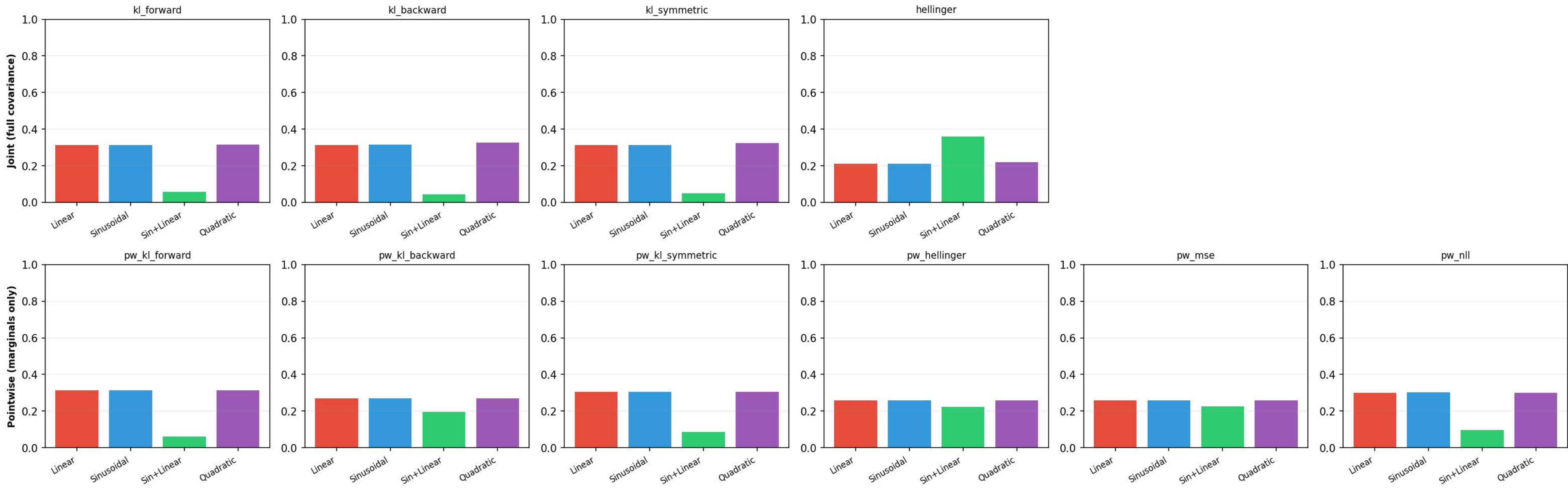
Joint vs Pointwise — Prior: vague — \tau \approx 1.0
