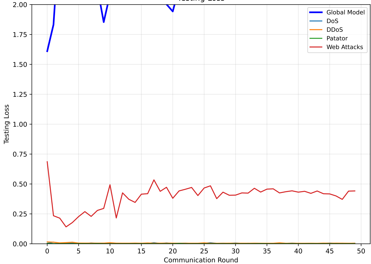
Testing Loss
