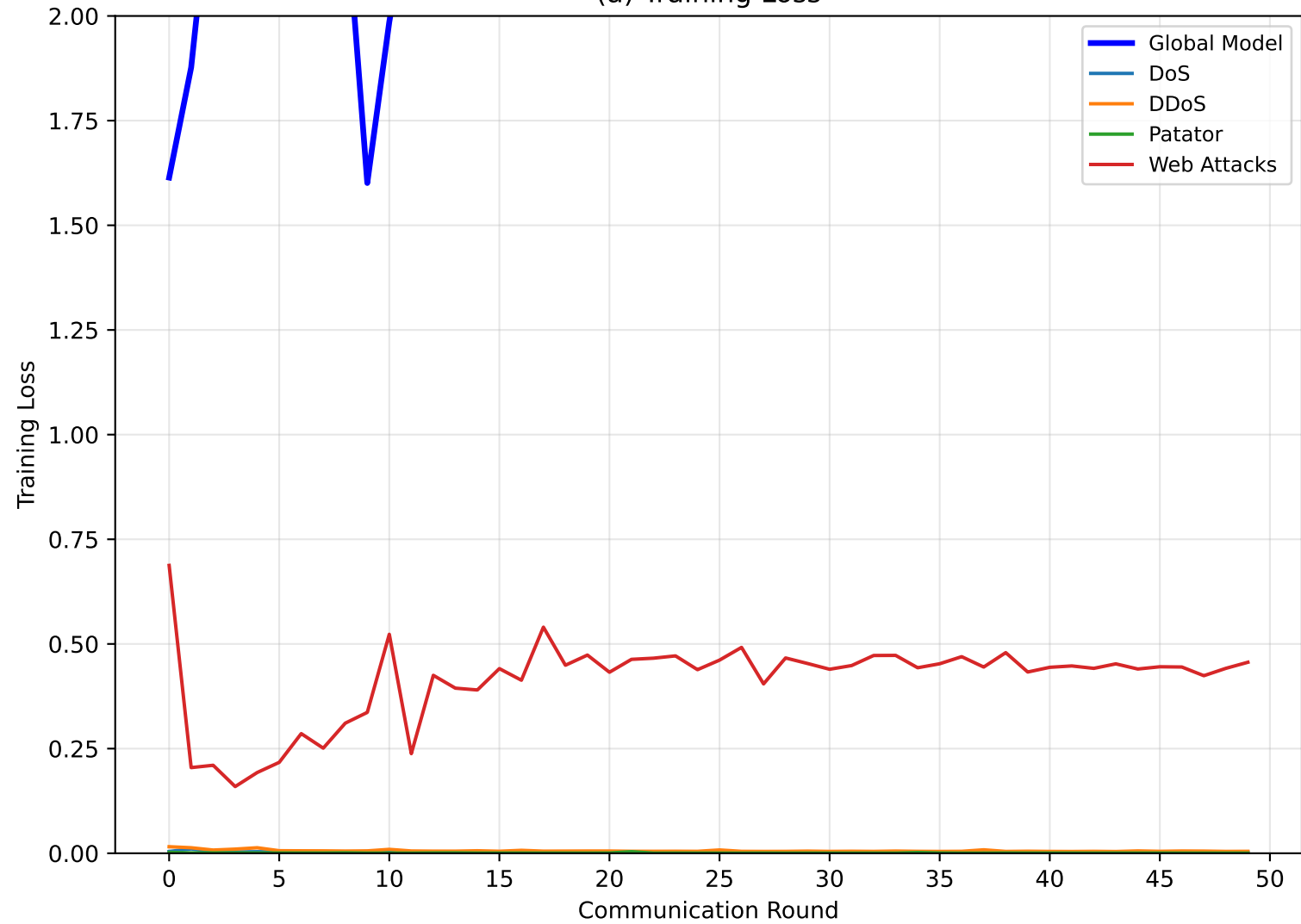
(a) Training Loss
