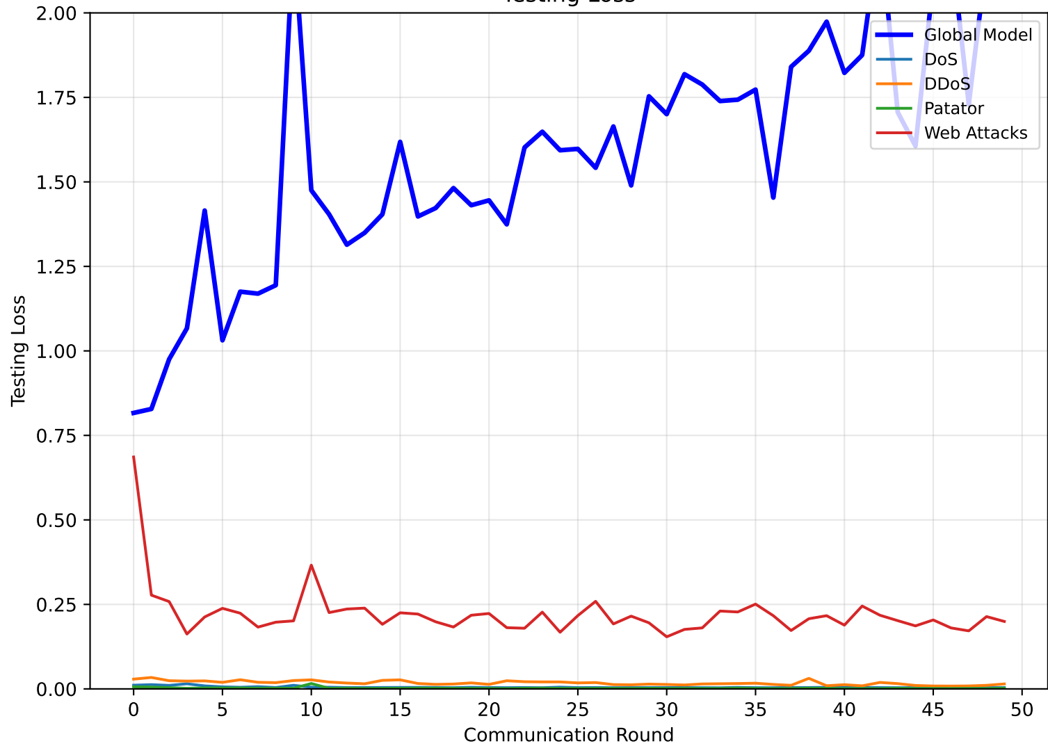
Testing Loss
