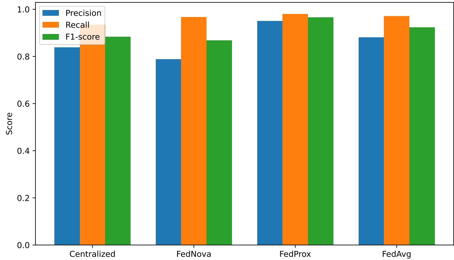
Model Accuracy
