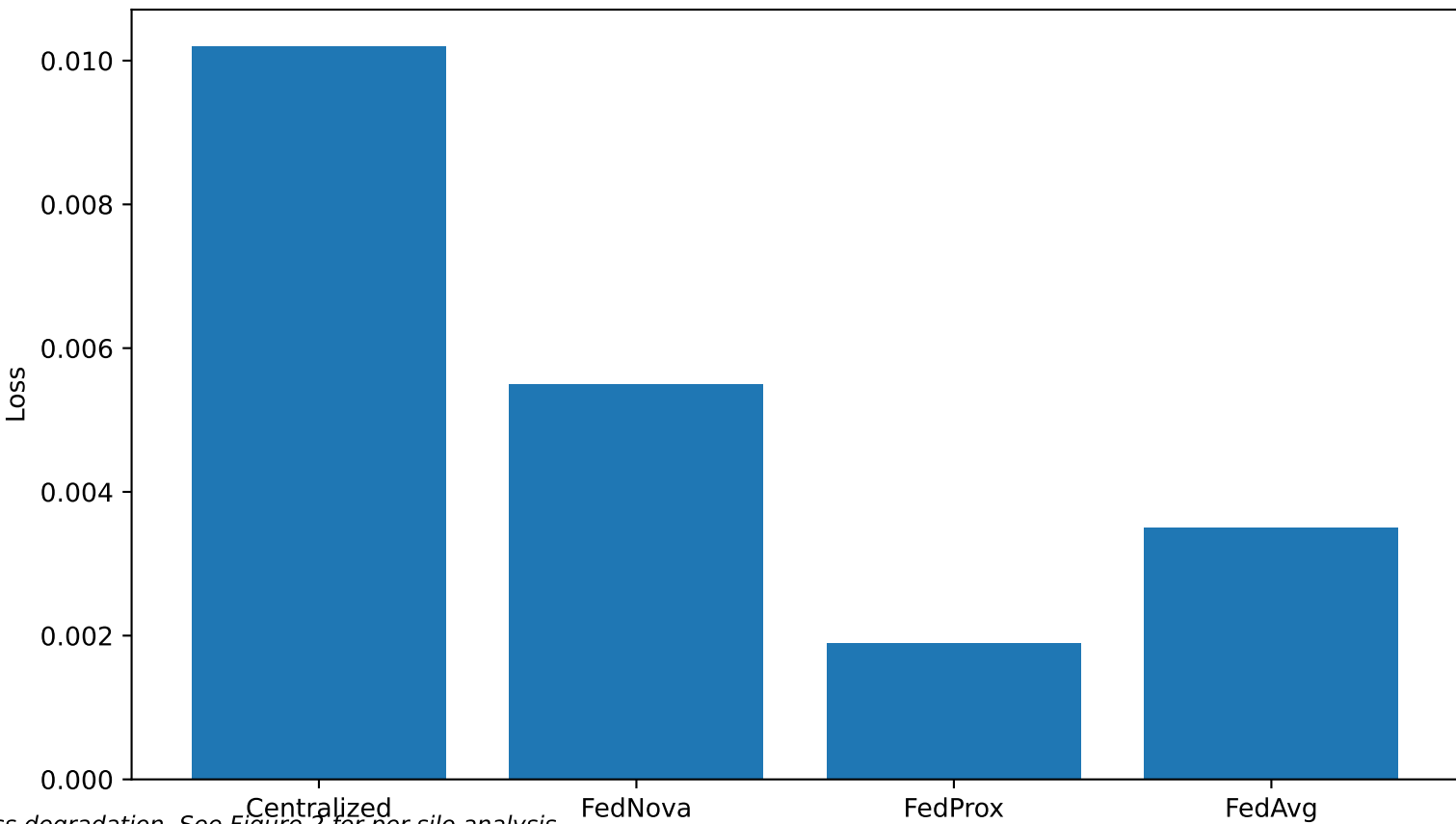
Test Loss
