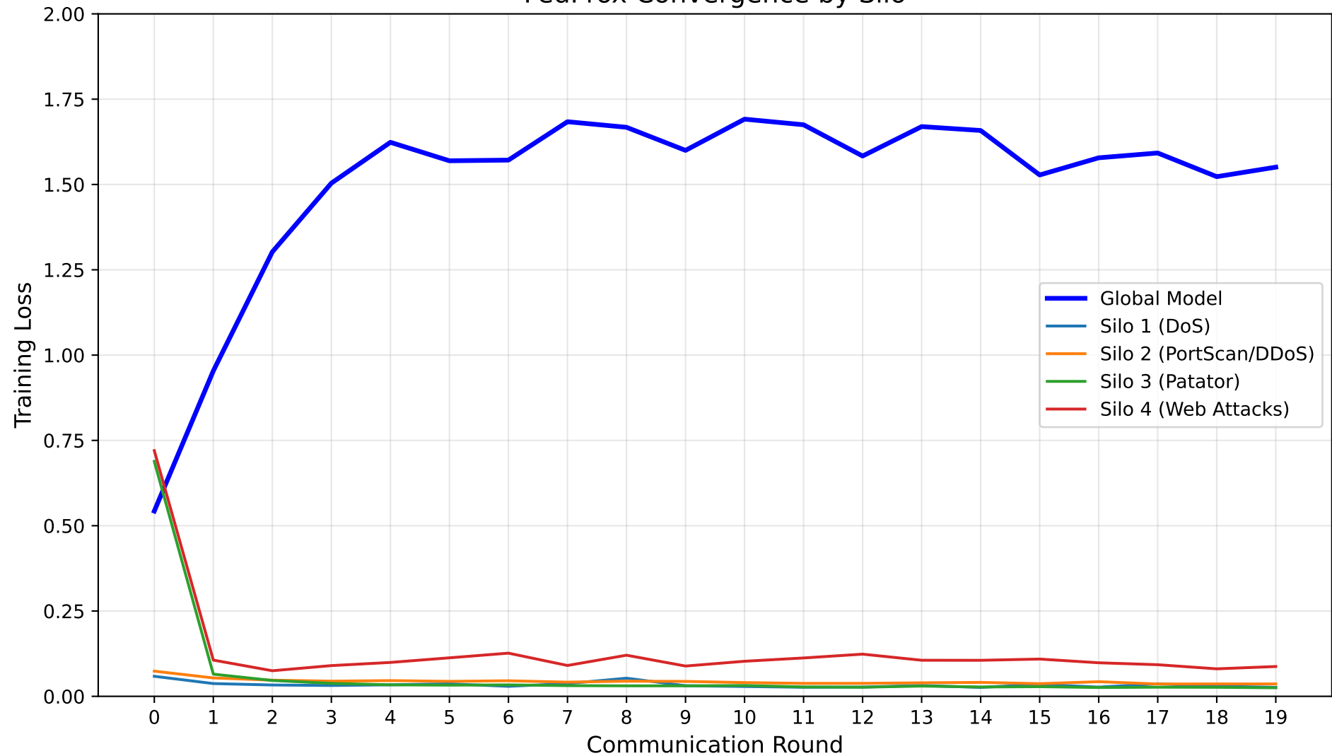
FedProx Convergence by Silo
