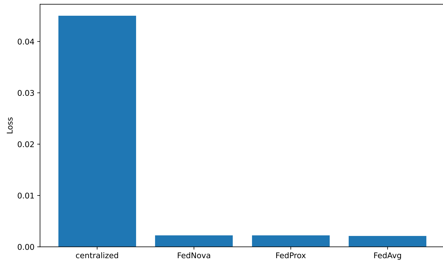
Test Loss
