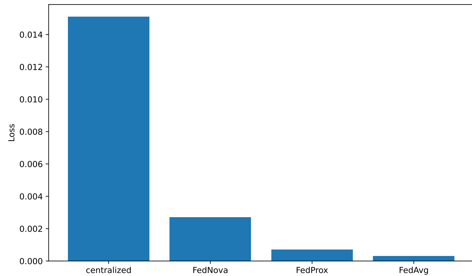
Test Loss
