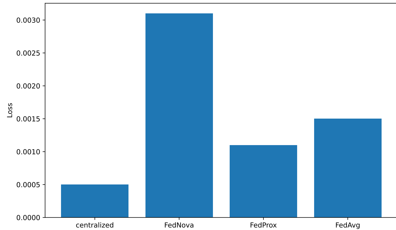
Test Loss
