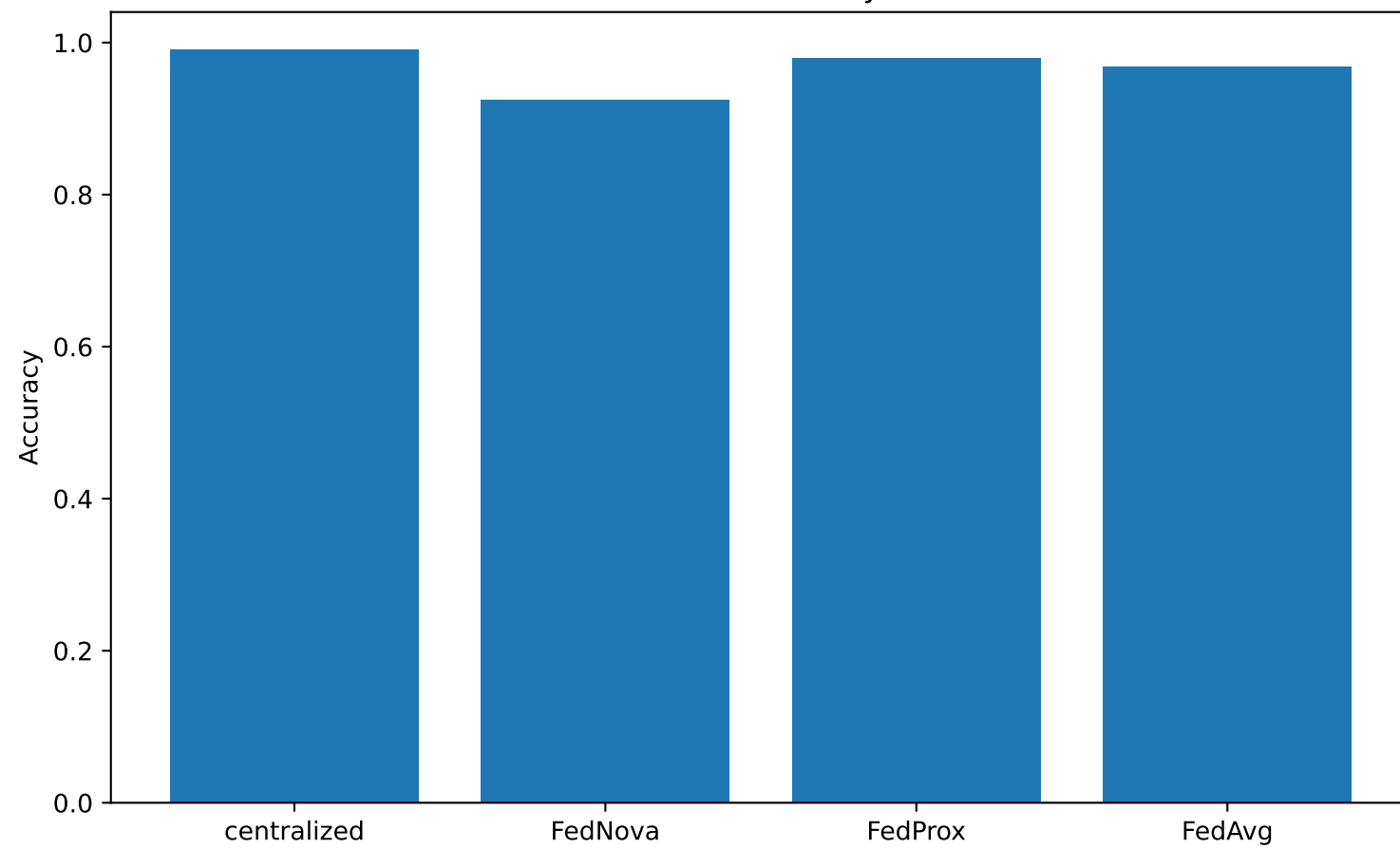
Model Accuracy
