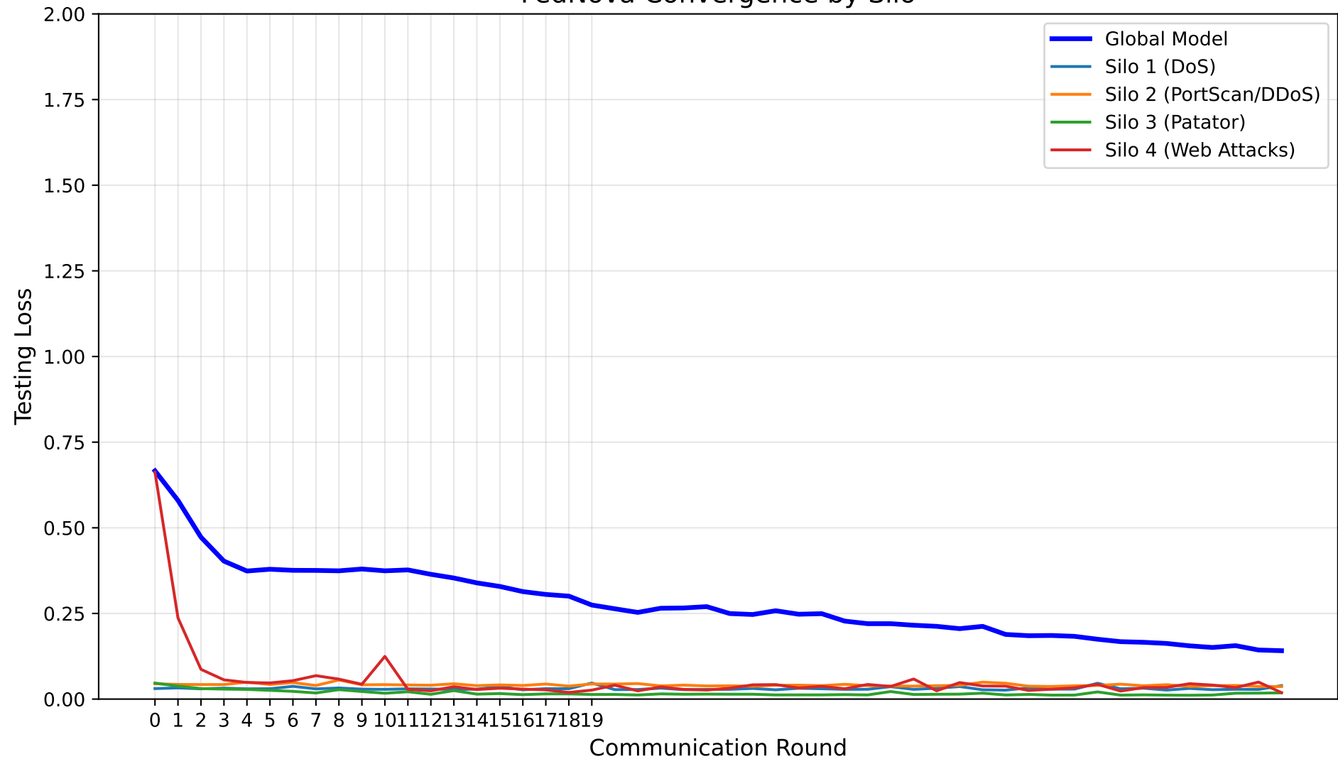
FedNova Convergence by Silo
