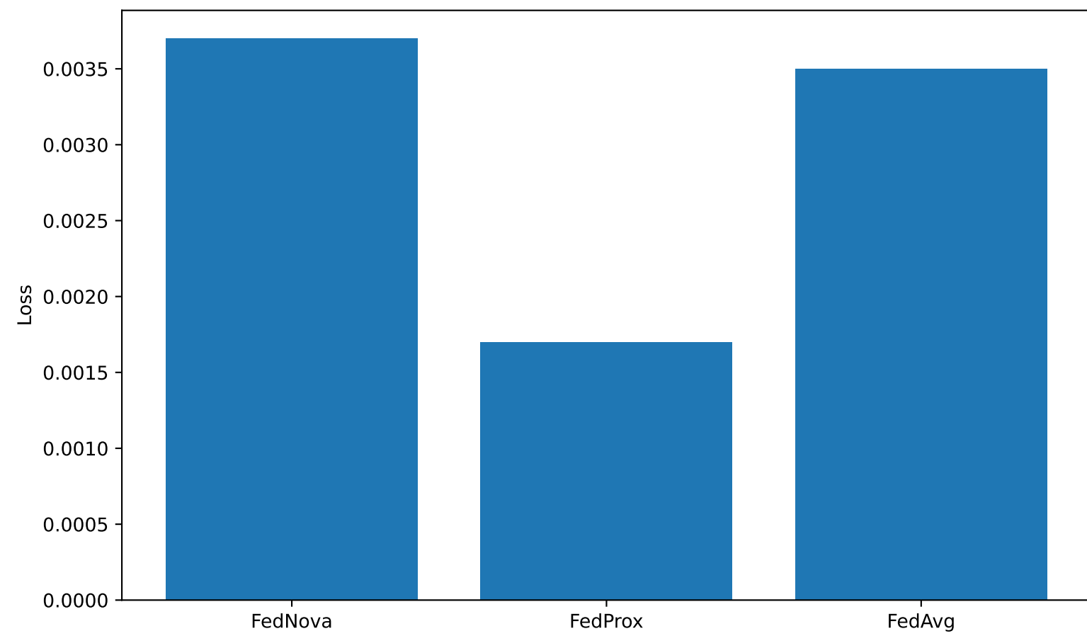
Test Loss
