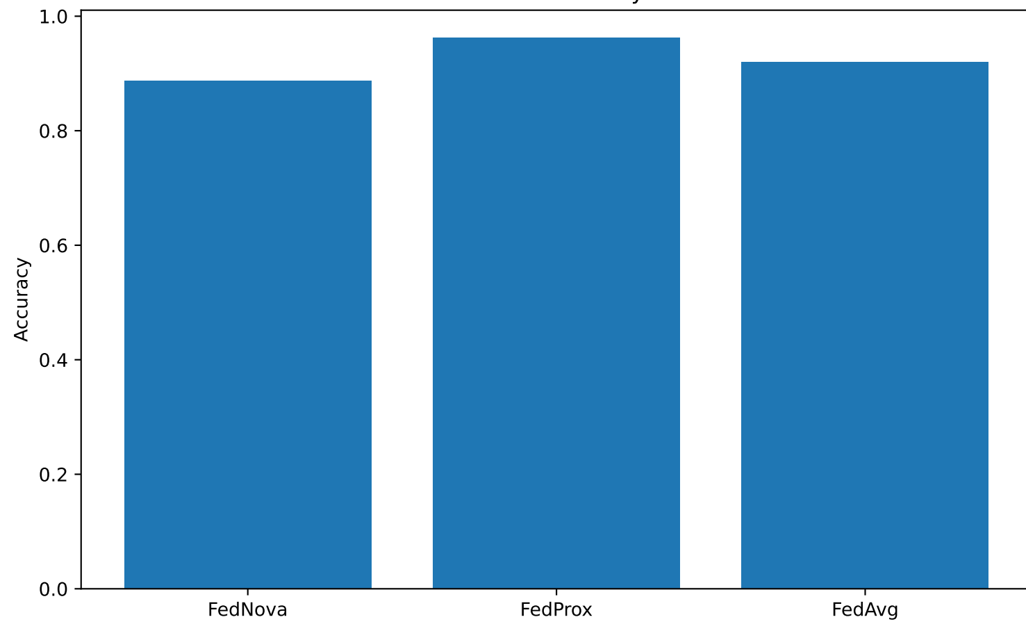
Model Accuracy
