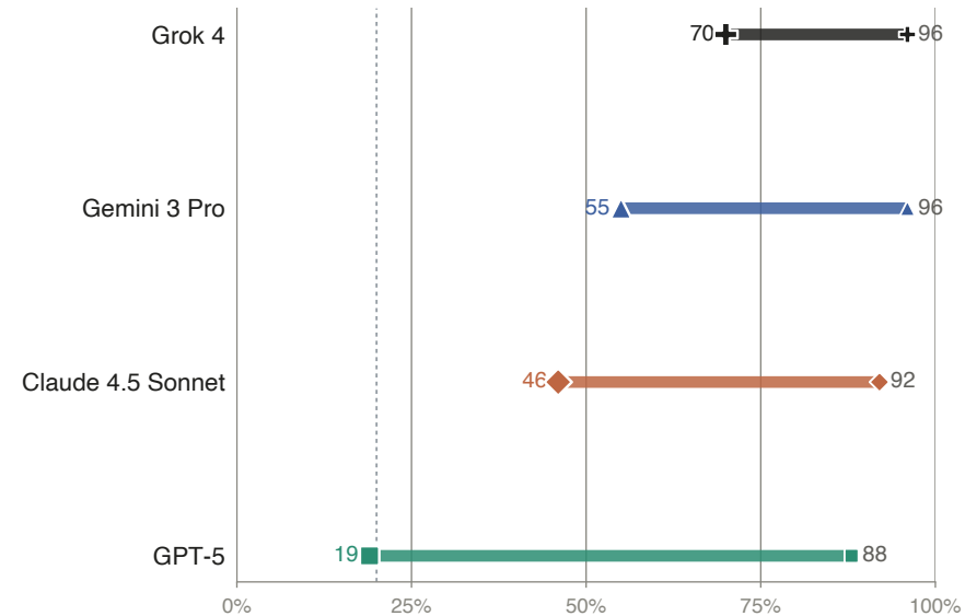
c Standard vs adversarial
