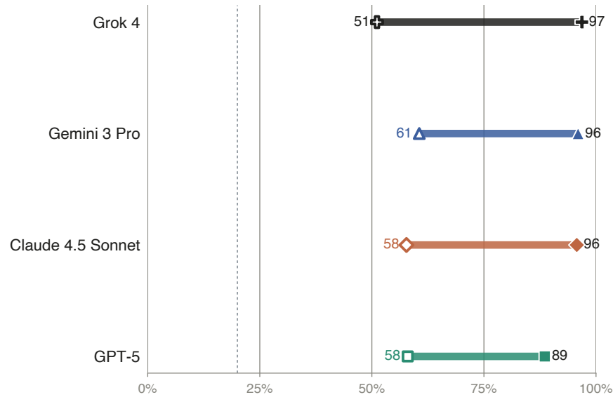
a Web-search ablation
