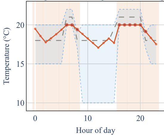
building 62 – indoor temperature (central opt)
