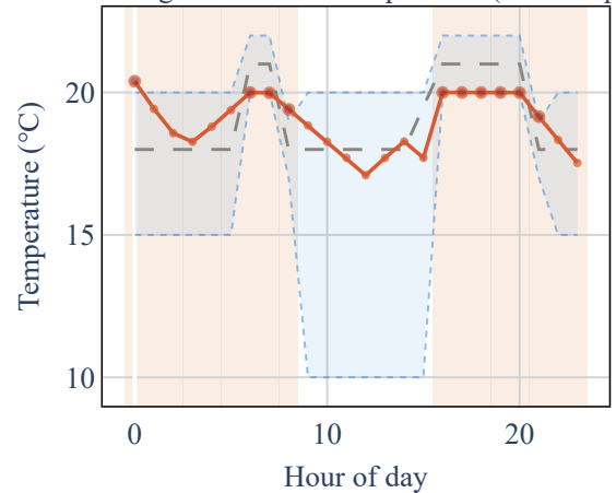
building 263 – indoor temperature (central opt)
