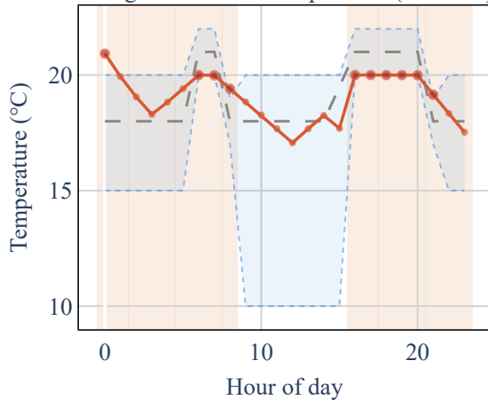
building 242 – indoor temperature (central opt)
