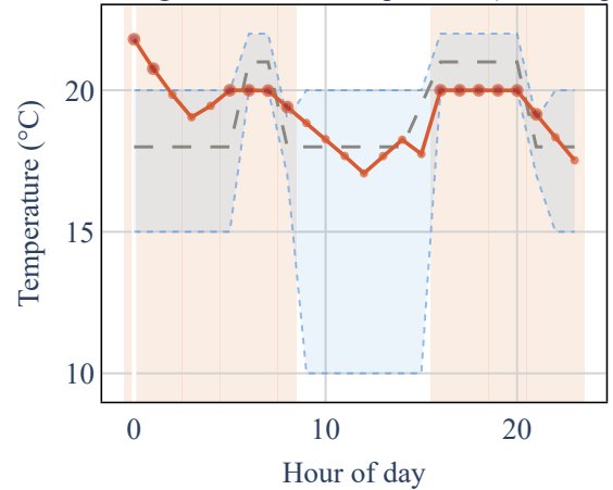
building 249 – indoor temperature (central opt)
