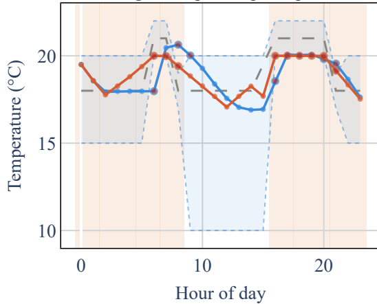
building 62 – open loop vs optimised
