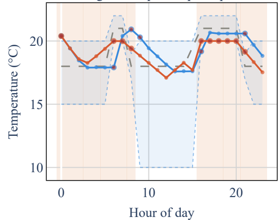
building 263 – open loop vs optimised
