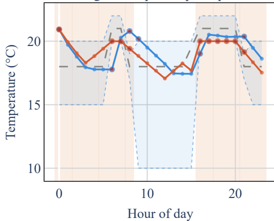
building 242 – open loop vs optimised
