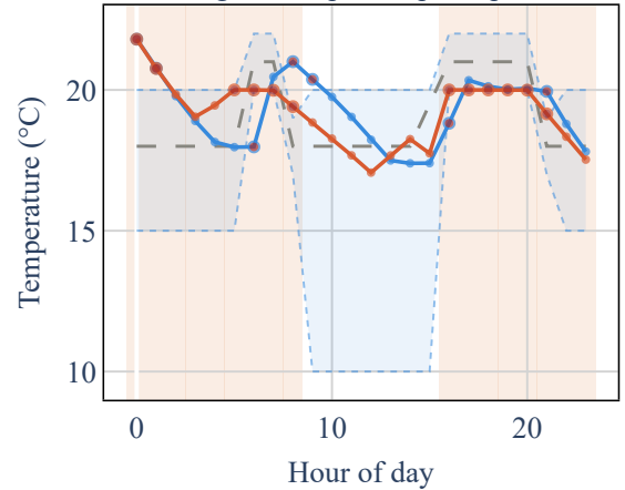
building 249 – open loop vs optimised
