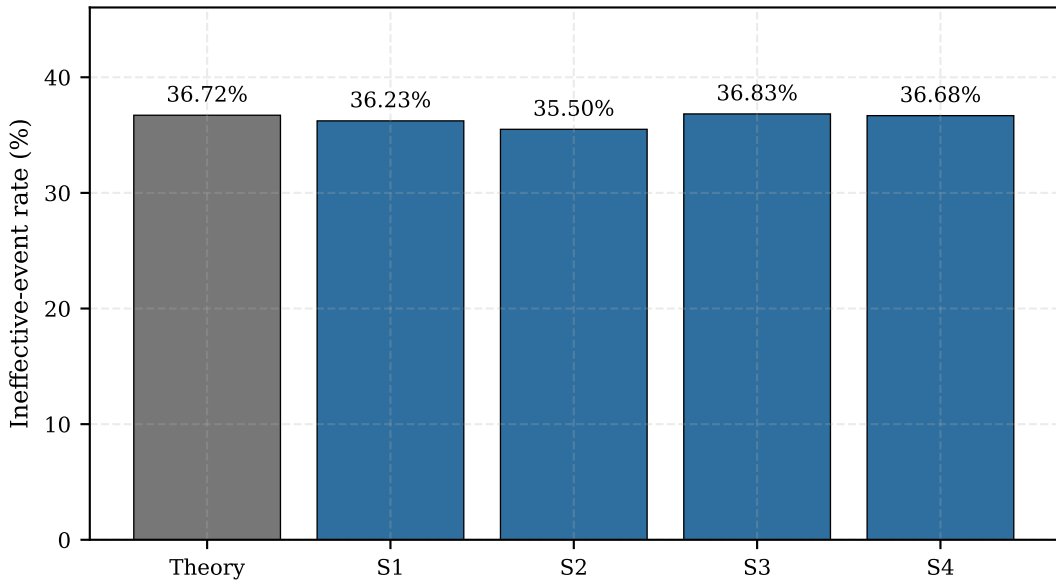
Theoretical and empirical ineffective-event rates
