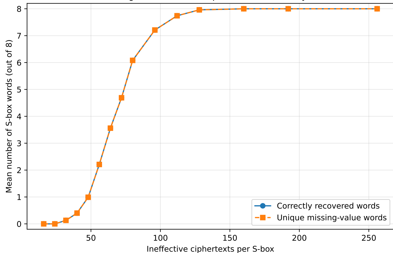
Progress toward complete SK28 recovery
