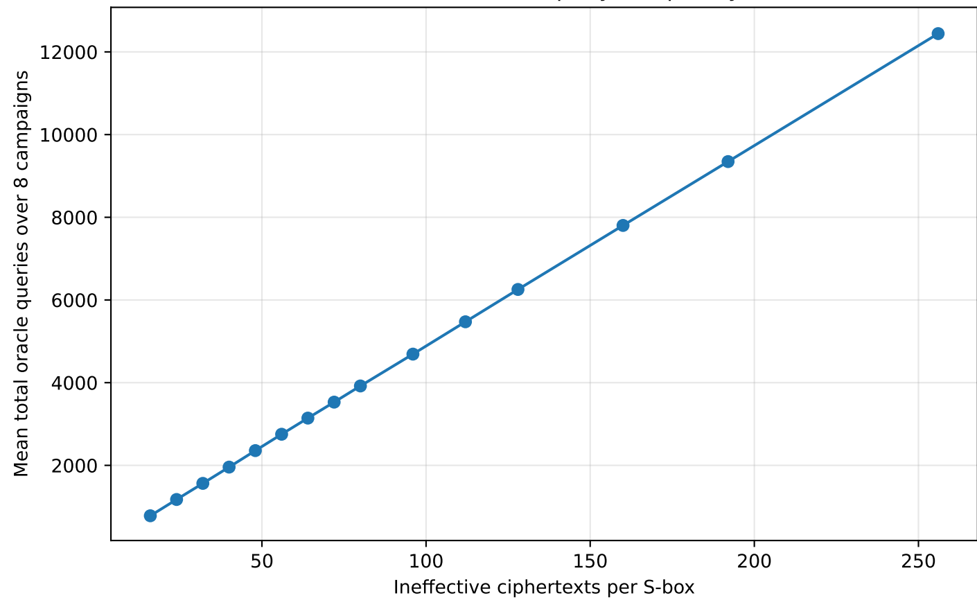
Scenario 1 oracle-query complexity
