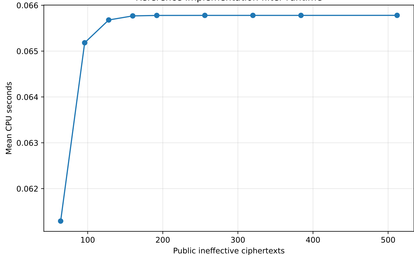
Reference implementation filter runtime
