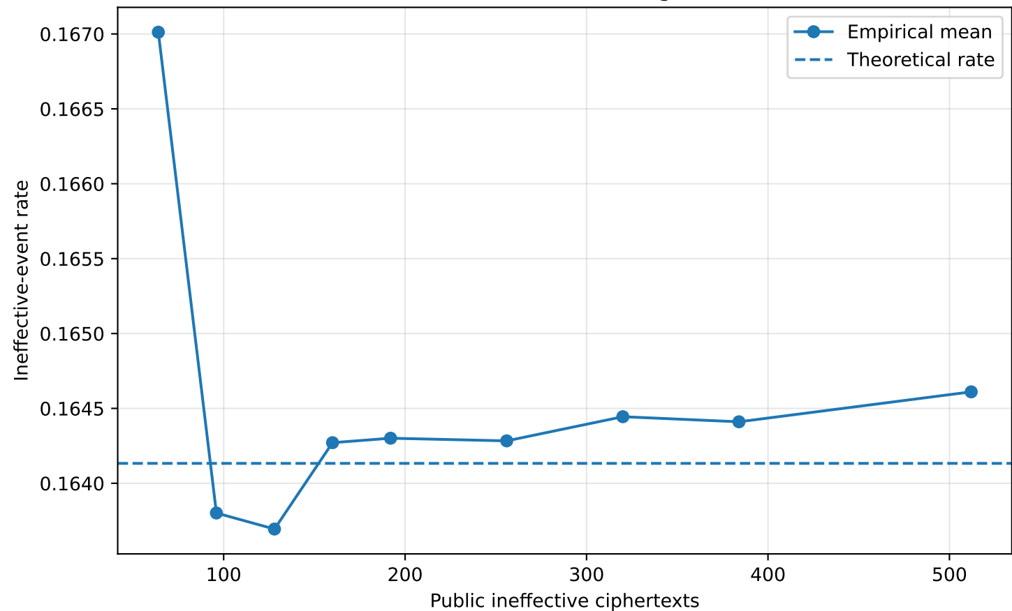
Ineffective-rate convergence
