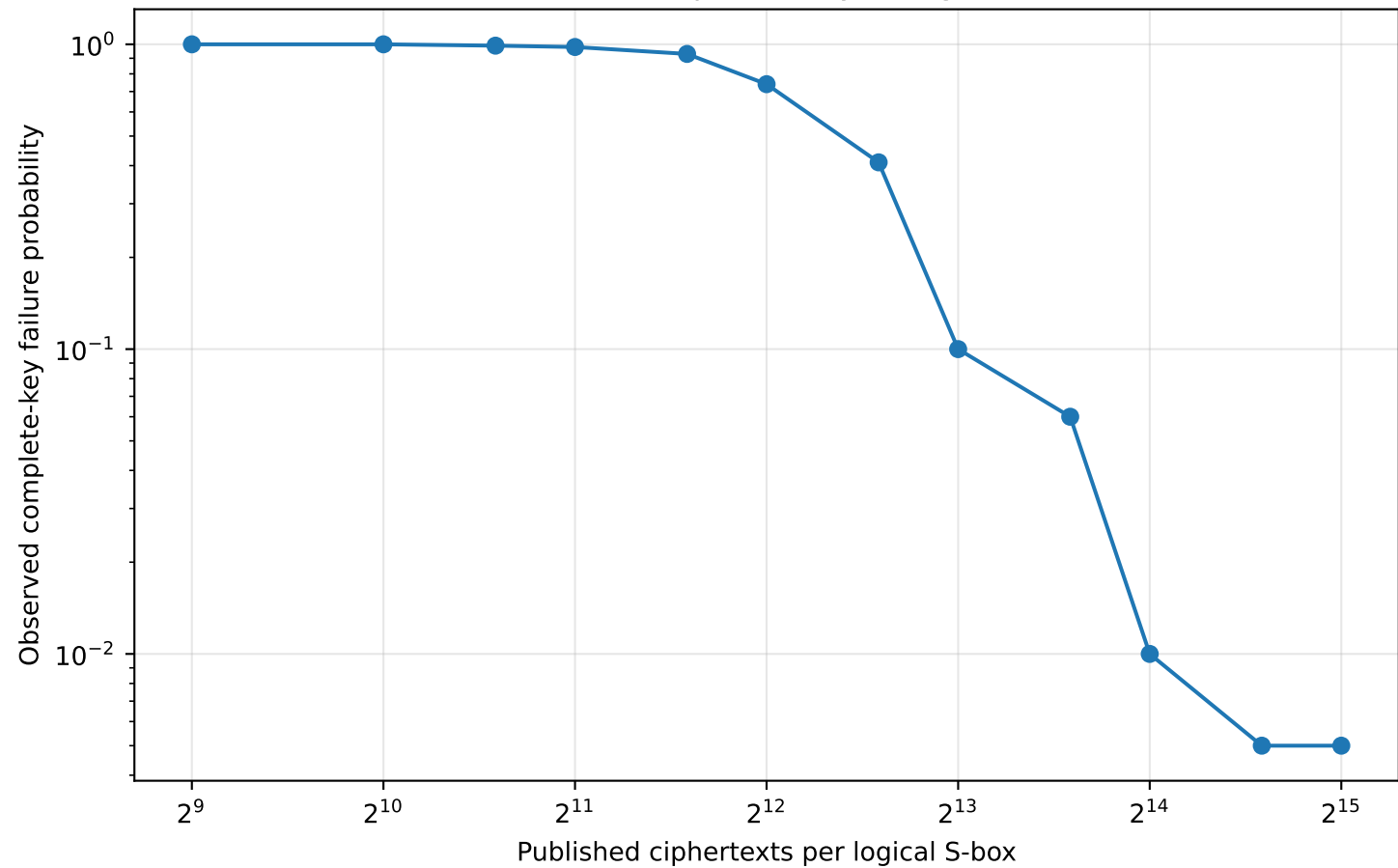
Residual failure probability of Algorithm 3
