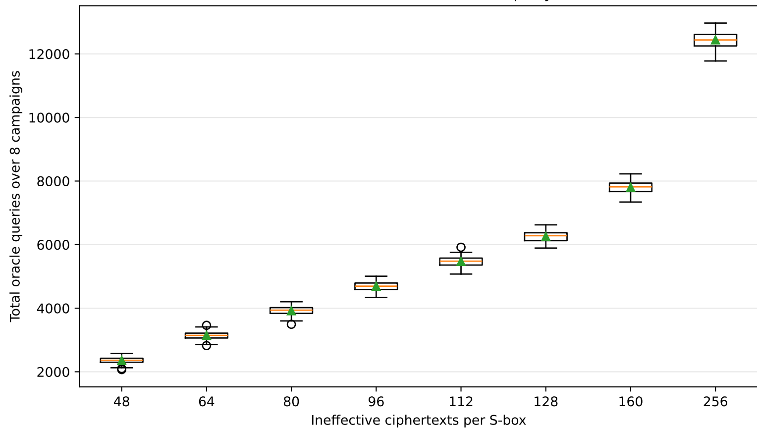
Distribution of Scenario 1 oracle-query cost
