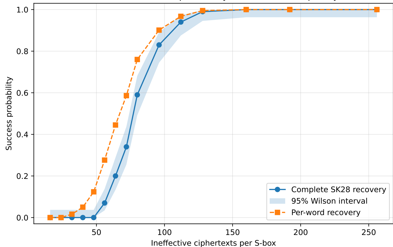
Scenario 1 success probability versus data complexity
