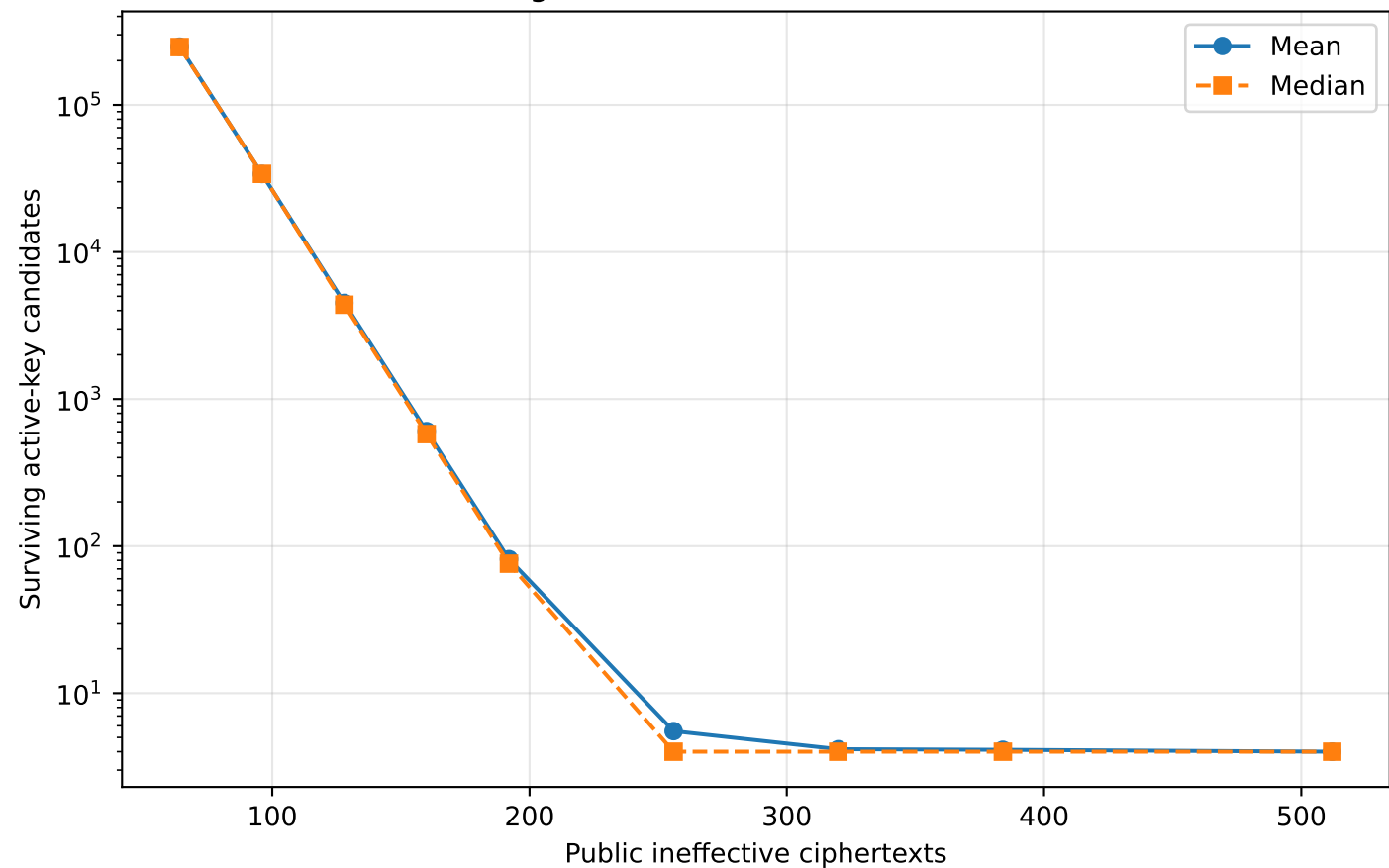
Algorithm-2 candidate reduction
