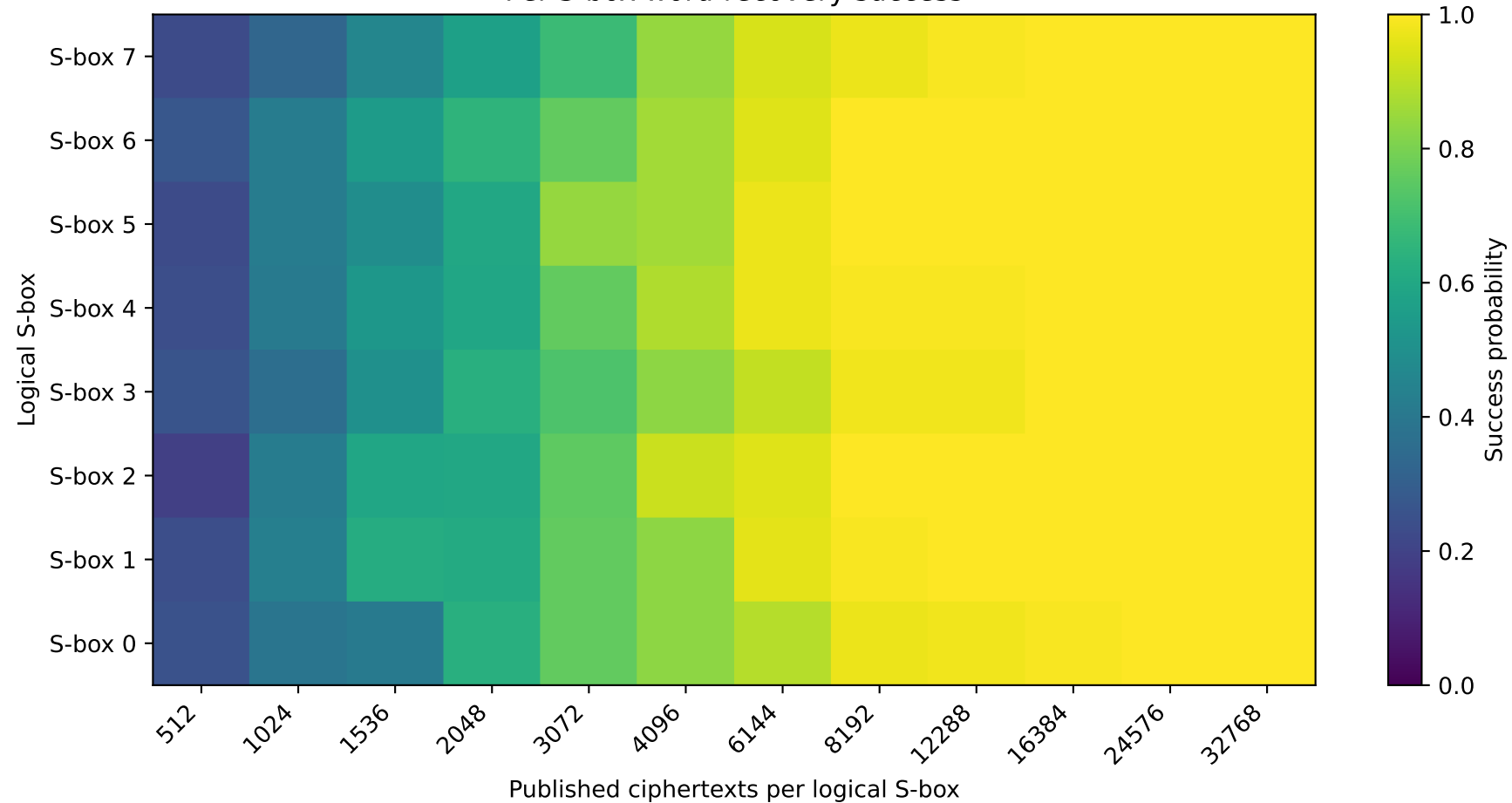
Per-S-box word-recovery success
