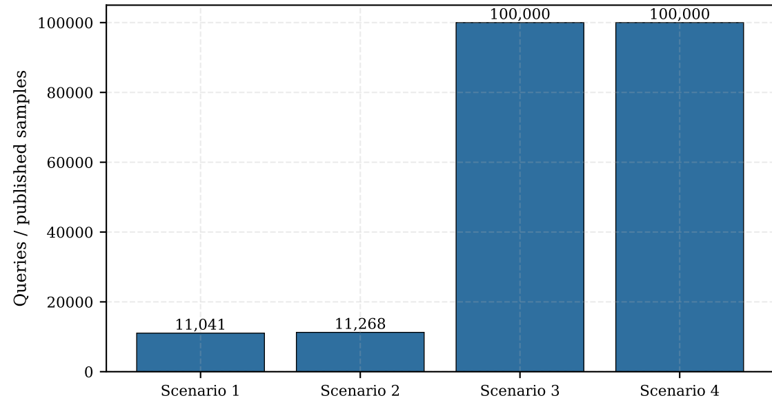
Observed data complexity
