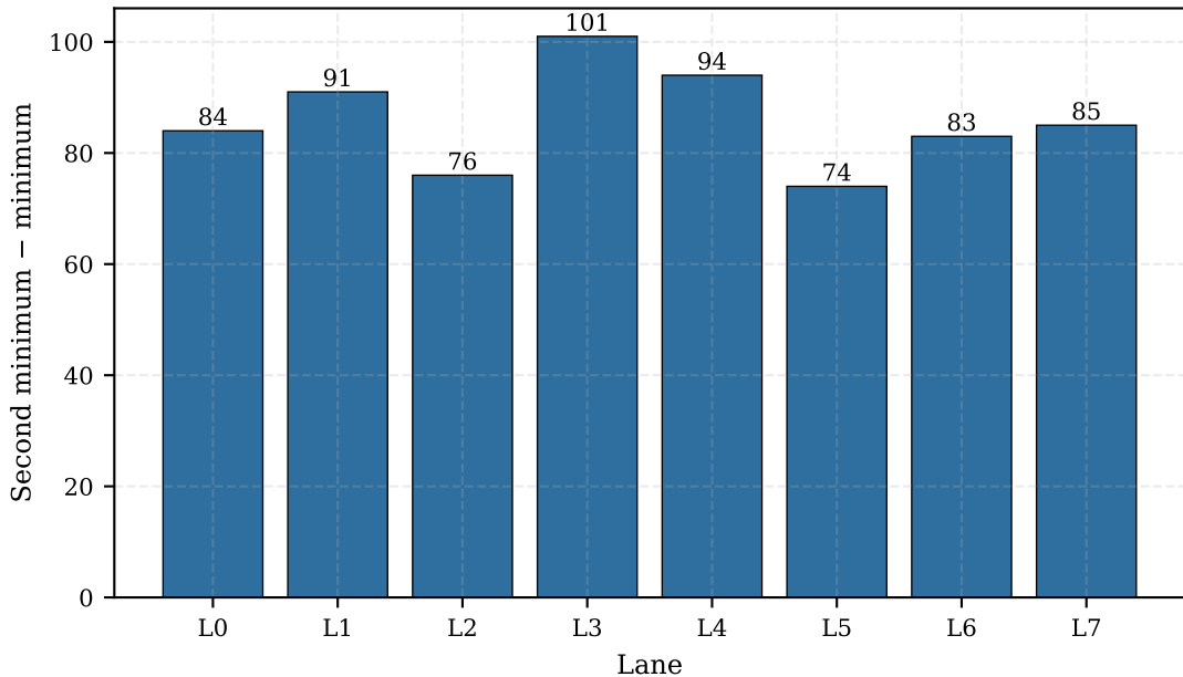
Scenario 3: statistical separation of the target bin
