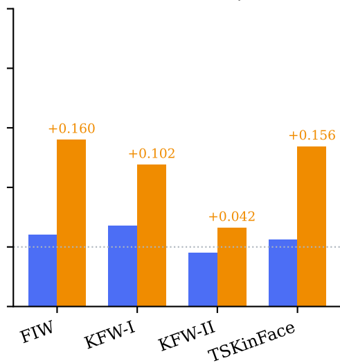
ArcFace \Delta=+0.115 , p=3e-07
