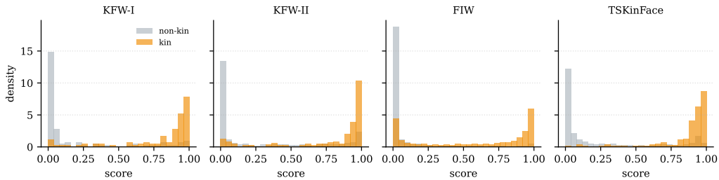
Figure 7: Kin and non-kin score distributions on the held-out fold of each corpus. The overlap, rather than any single summary statistic, is what the reported ROC-AUC measures.
