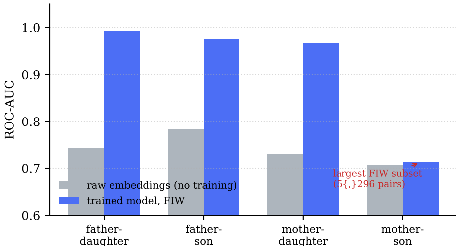
Per-relation difficulty, before and after training
