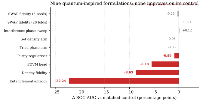
Fig. 11. Nine quantum-inspired formulations against classical controls matched for capacity or intent. None improves on its control; four are significantly worse. Bars are \Delta ROC-AUC in percentage points.
