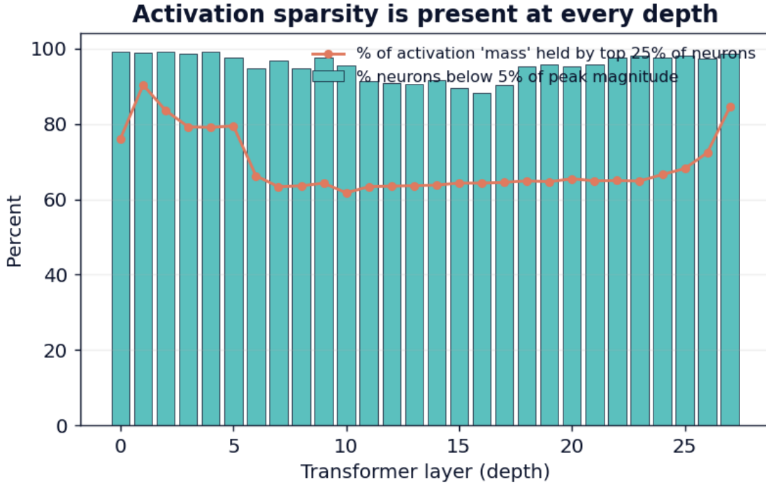
Figure 2. Activation sparsity at every transformer depth.
