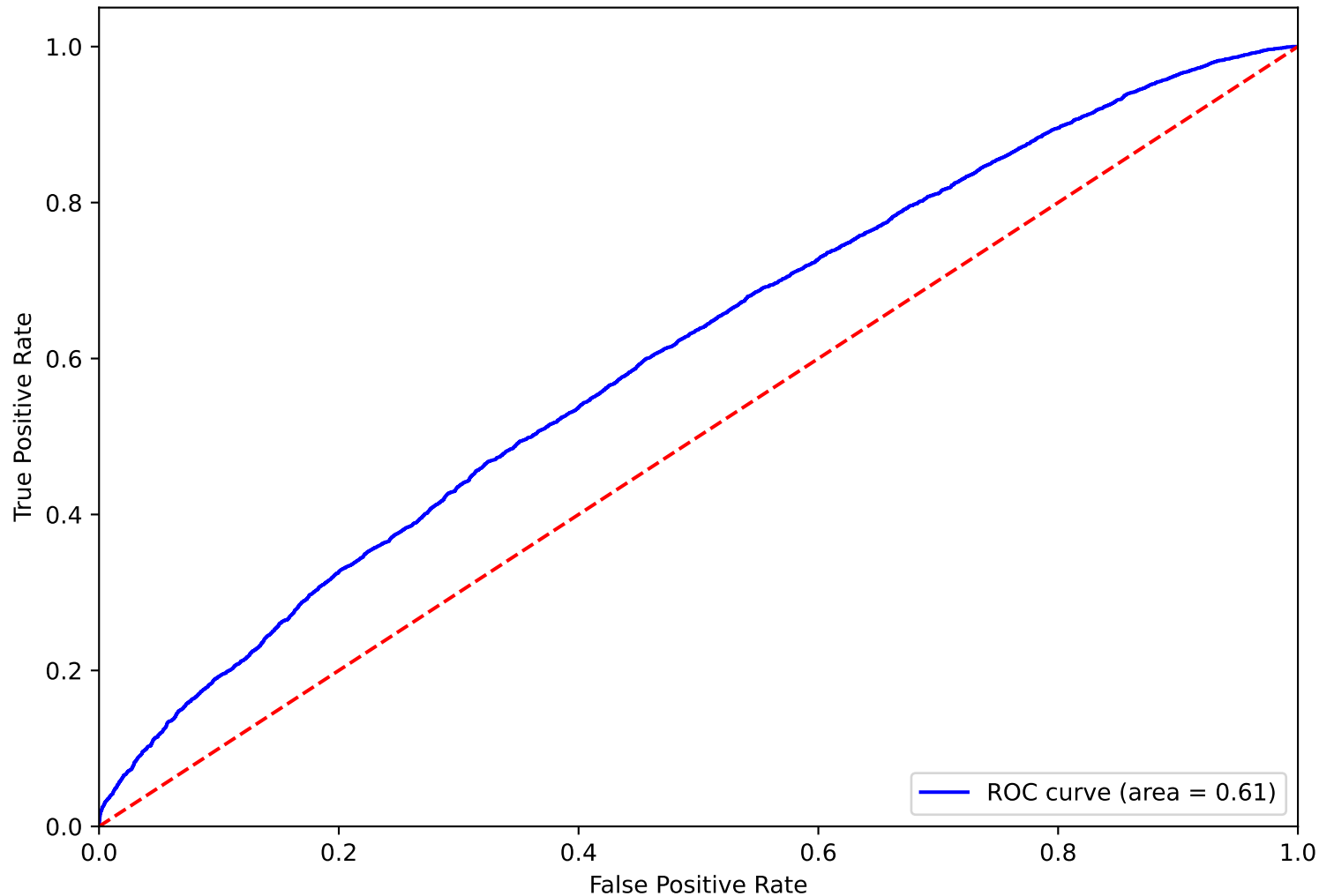
Receiver Operating Characteristic LightGBM Classifier on Bout-Level Outcomes
