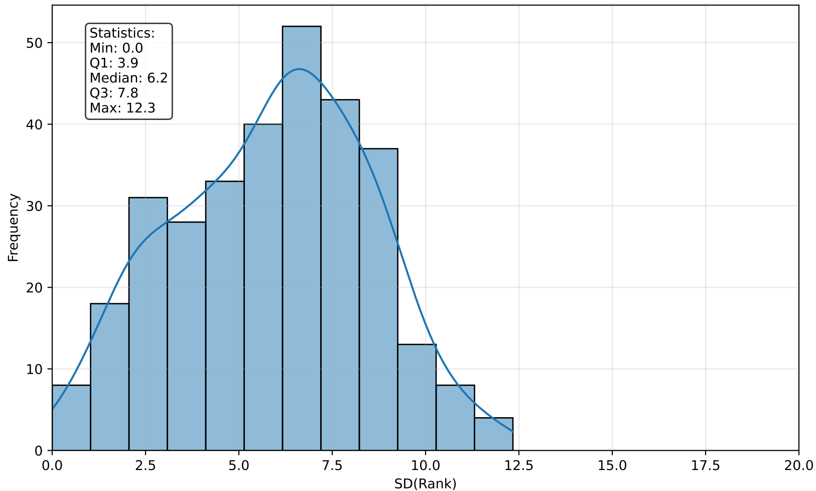
Career Rank Std. Dev. Distribution
