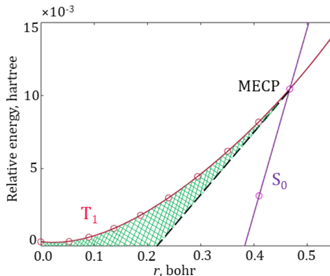
Figure 6.12. The fitted T_1 \rightarrow \text{MECP} \rightarrow S_0 reaction pathway. The circles mark the energies of the IRC geometries projected on the reaction coordinate r . Green area shows an increase in the tunneling barrier width compared to the linear model (dashed black line). The coefficients of the fitting polynomials ( f(x) = 0.092 x^4 - 0.121 x^3 + 0.093 x^2 - 0.004 x - 1.86 \times 10^{-6} and g(x) = 0.127 x - 0.048 ) are included in the NAST input file.
