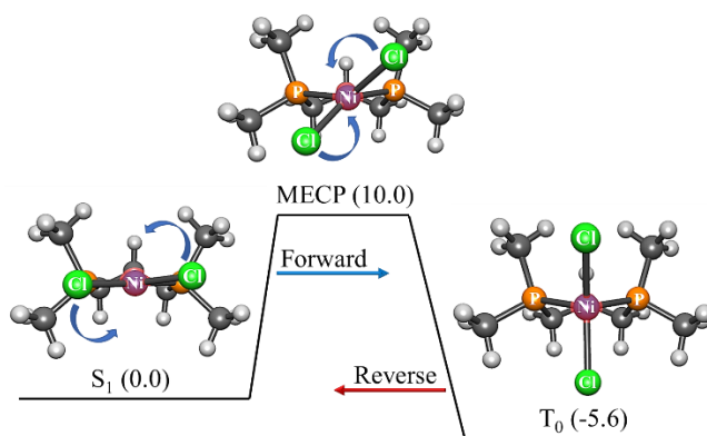
Figure 6.7. Reaction path of singlet-triplet isomerization of the \text{Ni(dpp)Cl}_2 model from square-planar to tetragonal geometry. The angles between the \text{Cl-Ni-Cl} and \text{P-Ni-P} planes are 6^\circ , 42^\circ and 90^\circ for the singlet, MECP, and triplet geometries, respectively. The benzene rings of \text{Ni(dpp)Cl}_2 are replaced with the methyl groups.
