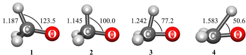
Figure 7.2. \text{CH}_3\text{O}^+ structures (1 \rightarrow 4) generated by displacements along the reaction coordinate normal mode at MECF and visualized by MacMolPlt.
