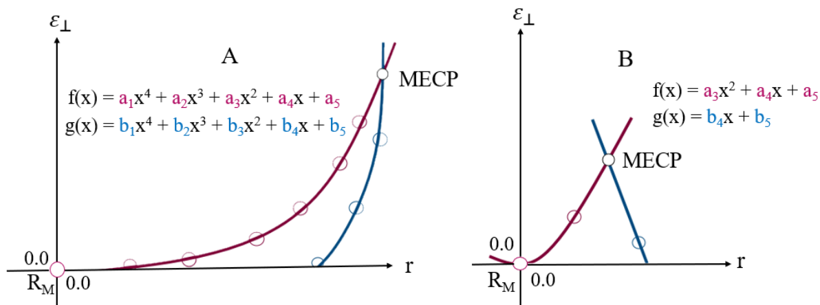
Figure 7.3. Examples of the fitted IRC paths along 1-D reaction coordinate r . R_M is the reactant minimum, \varepsilon_{\perp} is the energy perpendicular to the crossing seam. A) Sloped-type intersection; reactant and product points are fitted to a quartic polynomial. B) Peaked-type intersection; reactant and product points are fitted to a parabola and a line, respectively.
