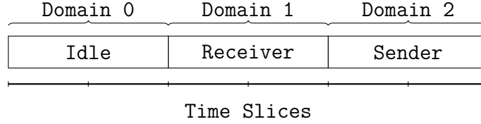
Figure 4: Timeline of the Blinky Domain Scheduling
