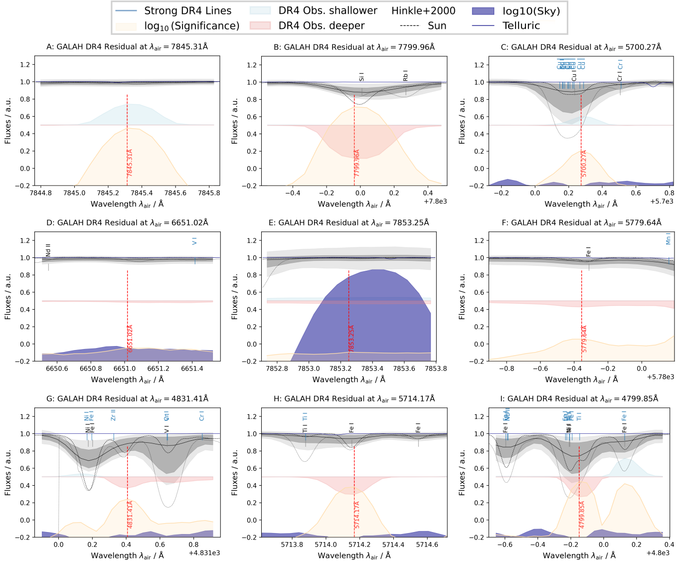
FIG. 4.— Representative significant residual regions and their adopted classifications. Panels A–I illustrate, respectively, candidate \log gf too high, \log gf too low, Line profile, Insignificant, Skyline, Interstellar, Unknown line, Known missing, and Unclear classifications. Each panel combines the GALAH residual statistics with relevant external diagnostics, including the Solar and Arcturus atlases, GALAH line-list entries, telluric absorption, and sky-emission measurements.
