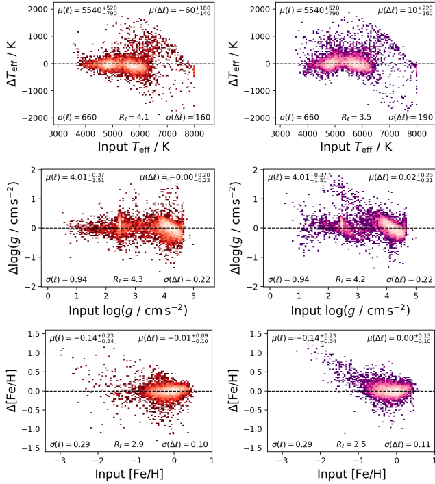
FIG. 9.— Cross-validated recovery of T_{\text{eff}} , \log g , and [\text{Fe}/\text{H}] using the 793 pixels excluded from the GALAH DR4 optimisation with Model M5 (left; red) and the 13134 pixels included in the optimisation with Model M6 (right; pink). Plotting conventions follow Fig. 5.
