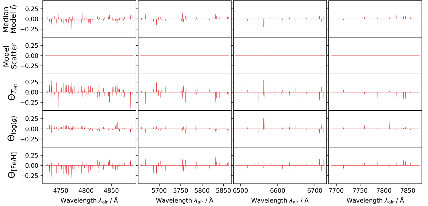
FIG. 10.— Selected coefficients across wavelength for Model M5 , using only the 793 wavelength pixels excluded from the GALAH DR4 optimisation. Lines show the median coefficient across the five cross-validation folds, and shaded regions show the full fold-to-fold range.
