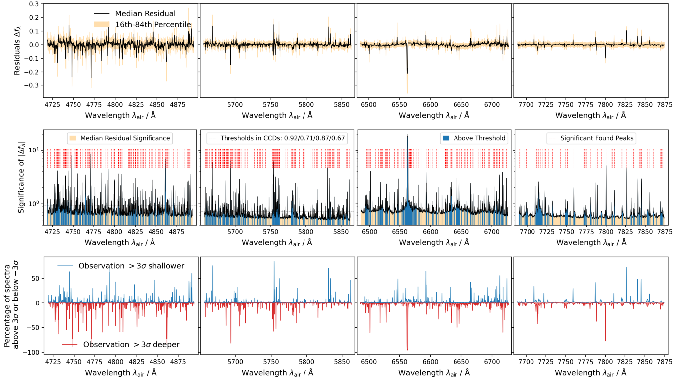
FIG. 3.— Residual statistics across the four GALAH wavelength bands. From top to bottom, the panels show the distribution of residual flux, the typical residual significance, and the fraction of the 7087 spectra for which the observed flux is significantly shallower (blue) or deeper (red) than the synthesis at more than 3\sigma . Columns correspond to the four HERMES CCD arms. An enlarged version of the middle panels can be found in our repository .
