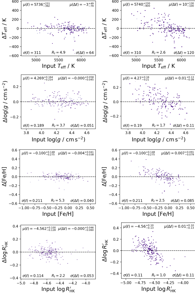
FIG. 7.— In-sample fit (left) and out-of-sample cross-validated recovery (right) of T_{\text{eff}} , \log g , [\text{Fe}/\text{H}] , and \log R'_{\text{HK}} with Model M4 for the 226 stars in the activity sample. The left panels show predictions from a model trained and evaluated on the complete sample and therefore do not provide an independent performance estimate. The right panels combine predictions for the left-out spectra from the five cross-validation folds. Plotting conventions follow Fig. 5.
