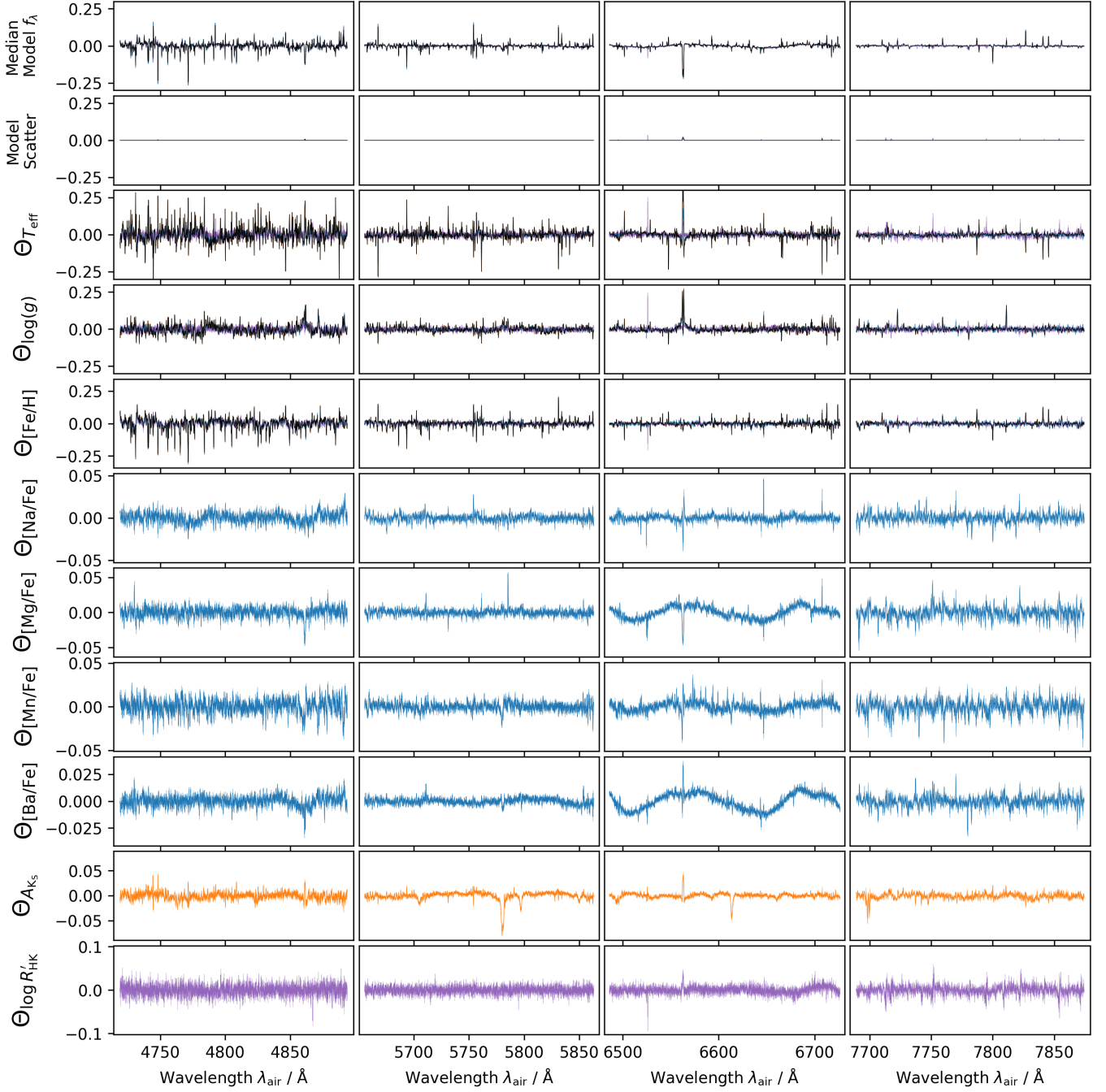
FIG. 6.— Selected coefficients across wavelength for Models M1, M2, M3, and M4. Lines show the median coefficient across the five cross-validation folds, and shaded regions show the full fold-to-fold range. Because the labels are internally centred and scaled, the coefficients describe the local residual response near the centre of each training-label distribution.
