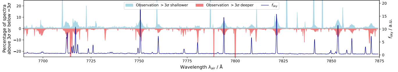
FIG. A1.— Comparison of the broad residual structure in the fourth GALAH wavelength band with observed sky-emission features. The agreement in wavelength supports the identification of these features as residuals associated with imperfect sky subtraction.
