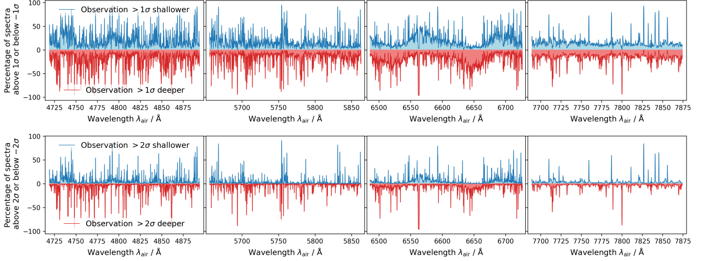
FIG. A2.— Fraction of spectra with observed flux significantly shallower or deeper than the synthesis at more than 1\sigma (top) and 2\sigma (bottom), shown across the four GALAH wavelength bands. The lower panels reproduce the significance threshold used in the bottom row of Fig. 3.
