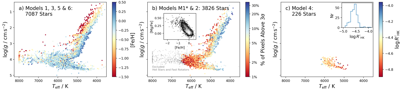
FIG. 2.— Stellar-label distributions of the three analysis samples in the T_{\text{eff}}-\log g plane. Left : the 7087-star baseline sample used for Models M1, M3, M5, and M6, colour-coded by [\text{Fe}/\text{H}] . Middle : the 3826-star abundance sample used for Models M1* and M2, coloured by the percentage of pixels with residual significance above 3\sigma ; excluded hot stars and fast rotators are shown as grey crosses, and the inset shows the selected stars in the [\text{Mg}/\text{Fe}]-[\text{Fe}/\text{H}] plane. Right : the 226-star activity sample used for Model M4, coloured by the activity indicator \log R'_{\text{HK}} from Zhang et al. (2024) with the \log R'_{\text{HK}} distribution in an inset.
