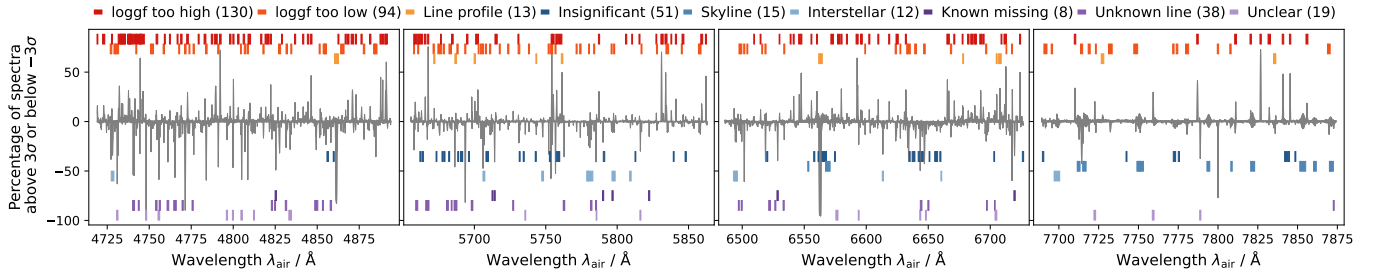
FIG. 11.— Classification map of the recurrent signed residual structure across the four GALAH wavelength bands. The underlying curves reproduce the fractions of baseline -sample spectra for which the observed flux is more than 3\sigma shallower or deeper than the synthesis, as shown in the bottom panels of Fig. 3. Short coloured bars mark the 380 catalogue regions and are grouped vertically by their adopted primary classification: candidate line-strength and Line profile mismatches in red and orange, Insignificant , Skyline , and Interstellar regions in blue, and missing, unidentified, or ambiguous features in purple. The vertical offsets are categorical and carry no quantitative meaning; the horizontal bar widths are proportional to the fitted residual-region widths.
