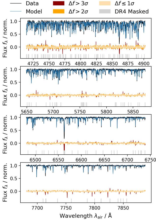
FIG. 1.— Example GALAH DR4 spectrum of the red giant 2MASS J22084160+0607286 (subject_id 170710003201361). Black and blue lines show the observed continuum-normalised spectrum and the best-fitting DR4 synthesis, respectively, across the four HERMES CCD arms. Shaded regions show the residual flux, with darker shades indicating larger significance relative to the reported flux uncertainty. Grey bands mark wavelength regions excluded from the DR4 optimisation.
