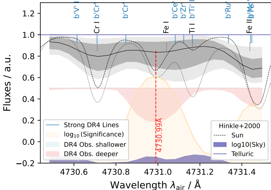
GALAH DR4 Residual at \lambda_{\text{air}} = 4730.99\text{\AA}
