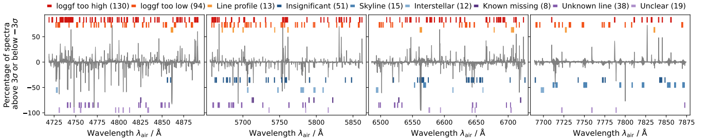
FIG. 13.— Classification map of the recurrent signed residual structure across the four GALAH wavelength bands. The underlying curves reproduce the fractions of baseline -sample spectra for which the observed flux is more than 3\sigma shallower or deeper than the synthesis, as shown in the bottom panels of Fig. 5. Short coloured bars mark the 380 catalogue regions and are grouped vertically by their adopted primary classification: candidate line-strength and Line profile mismatches in red and orange, Insignificant , Skyline , and Interstellar regions in blue, and missing, unidentified, or ambiguous features in purple. The vertical offsets are categorical and carry no quantitative meaning; the horizontal bar widths are proportional to the fitted residual-region widths.
