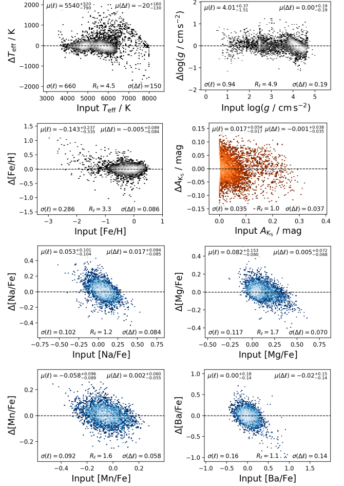
FIG. 7.— Cross-validated recovery differences, \Delta \ell = \ell_{\text{Cannon}} - \ell_{\text{reference}} , as a function of the reference labels for Models M1 (grey), M2 (blue), and M3 (orange). From top left to bottom right, the panels show T_{\text{eff}} , \log g , [\text{Fe}/\text{H}] , A_{K_S} , [\text{Na}/\text{Fe}] , [\text{Mg}/\text{Fe}] , [\text{Mn}/\text{Fe}] , and [\text{Ba}/\text{Fe}] . Dashed lines mark \Delta \ell = 0 . Annotations give the 16th, 50th, and 84th percentiles of the label and recovery distributions and the label-recovery ratio R_\ell . Equal axis scaling in label units allows the recovery scatter to be compared directly with the label spread.
