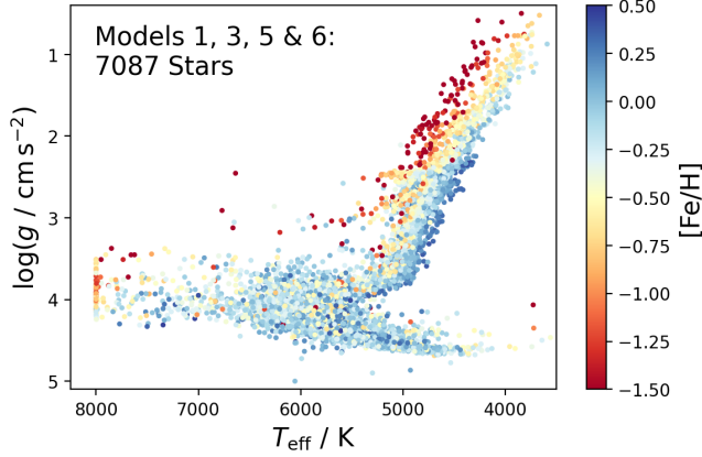
FIG. 2.— Distribution of the baseline sample used for Models M1, M3, M5, and M6 in the T_{\text{eff}} – \log g plane, colour-coded by [\text{Fe}/\text{H}] . The sample spans a broad range of stellar parameters and evolutionary stages.
