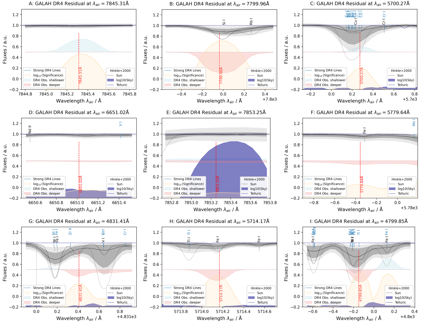
FIG. 6.— Representative significant residual regions and their adopted classifications. Panels A–I illustrate, respectively, candidate \log gf too high, \log gf too low, Line profile, Insignificant, Skyline, Interstellar, Unknown line, Known missing, and Unclear classifications. Each panel combines the GALAH residual statistics with relevant external diagnostics, including the Solar and Arcturus atlases, GALAH line-list entries, telluric absorption, and sky-emission measurements.
