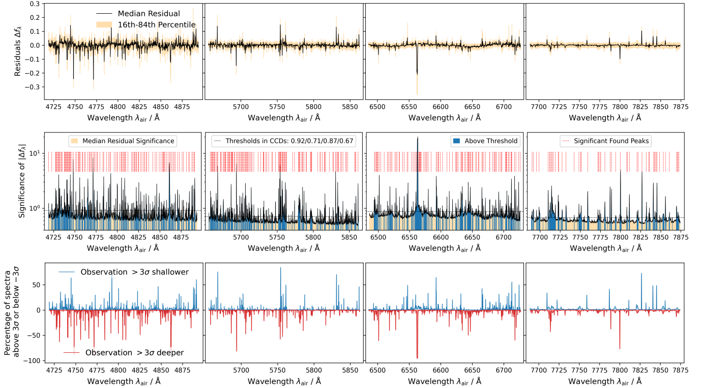
Fig. 5.— Residual statistics across the four GALAH wavelength bands. From top to bottom, the panels show the distribution of residual flux, the typical residual significance, and the fraction of the 7087 spectra for which the observed flux is significantly shallower (blue) or deeper (red) than the synthesis at more than 3\sigma . Columns correspond to the four HERMES CCD arms. An enlarged version of the middle panels can be found in our repository .
