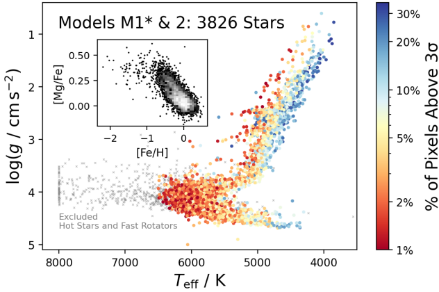
FIG. 3.— Distribution of the 3826 stars in the abundance sample used for Models M1* and M2 in the T_{\text{eff}}\text{--}\log g plane, colour-coded by the percentage of pixels with residuals above 3\sigma . Hot stars and fast rotators excluded from this sample are shown as grey crosses. The inset shows the selected stars in the [\text{Mg}/\text{Fe}]\text{--}[\text{Fe}/\text{H}] plane.
