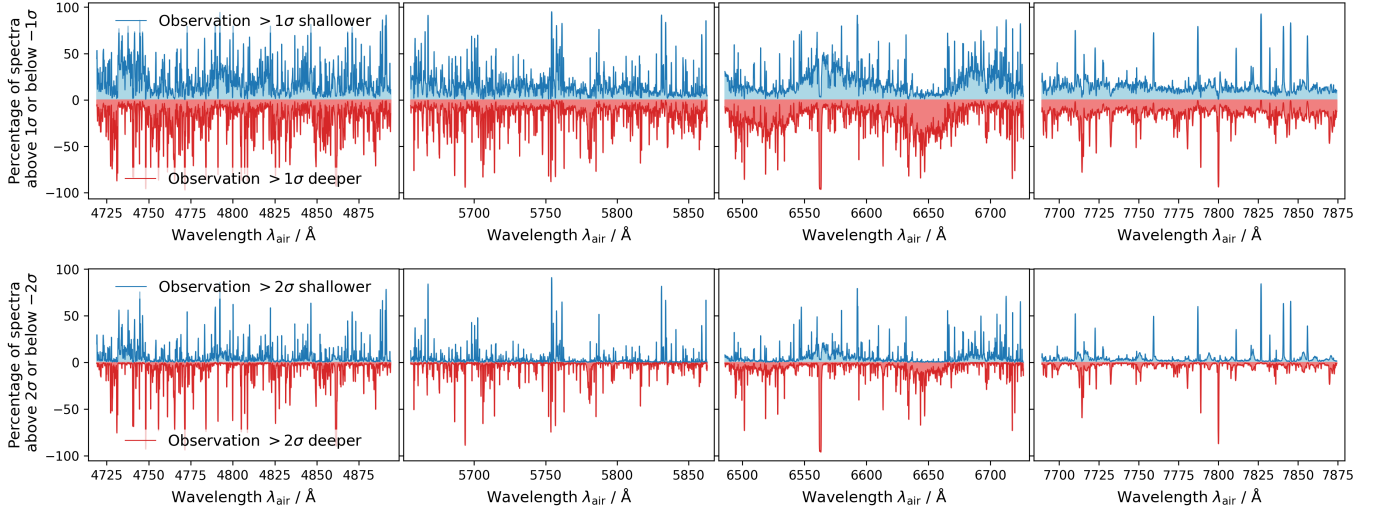
FIG. A1.— Fraction of spectra with observed flux significantly shallower or deeper than the synthesis at more than 1\sigma (top) and 2\sigma (bottom), shown across the four GALAH wavelength bands. The lower panels reproduce the significance threshold used in the bottom row of Fig. 5.
