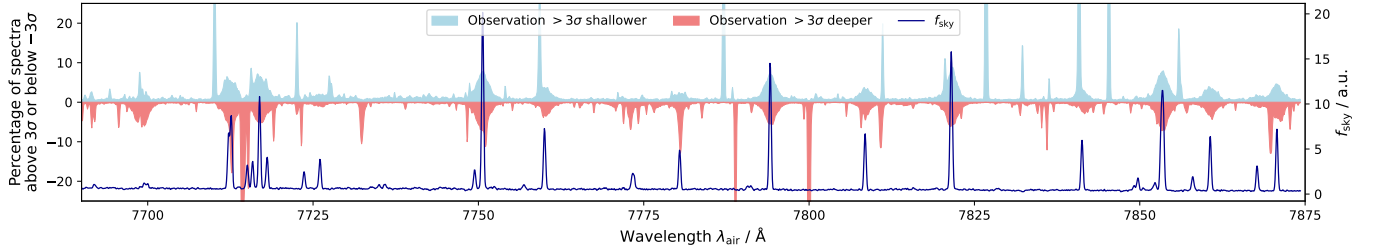
FIG. A2.— Comparison of the broad residual structure in the fourth GALAH wavelength band with observed sky-emission features. The agreement in wavelength supports the identification of these features as residuals associated with imperfect sky subtraction.
