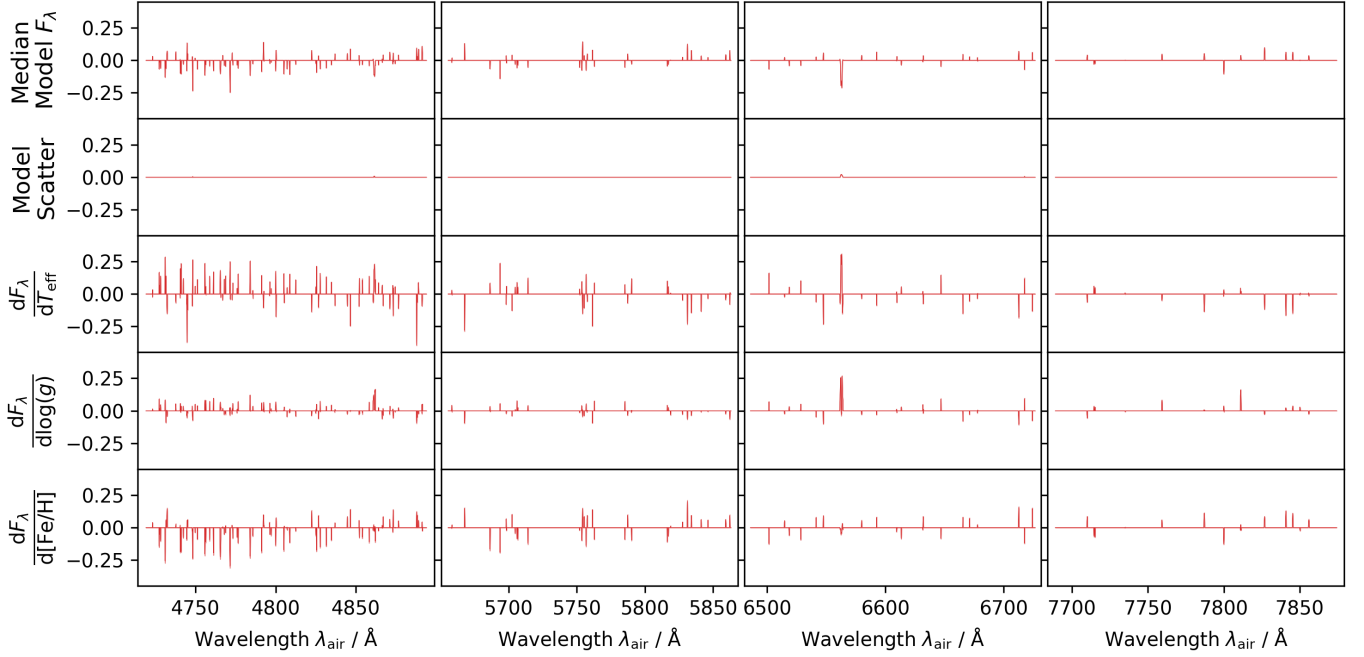
FIG. 12.— Selected coefficients across wavelength for Model M5 , using only the 793 wavelength pixels excluded from the GALAH DR4 optimisation. Lines show the median coefficient across the five cross-validation folds, and shaded regions show the full fold-to-fold range.
