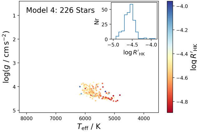
FIG. 4.— Distribution of the activity sample used for Model M4 in the T_{\text{eff}}\text{--}\log g plane, colour-coded by the activity indicator \log R'_{\text{HK}} from Zhang et al. (2024). The sample is restricted to dwarf stars with measured activity indices. The inset shows the distribution of \log R'_{\text{HK}} .
