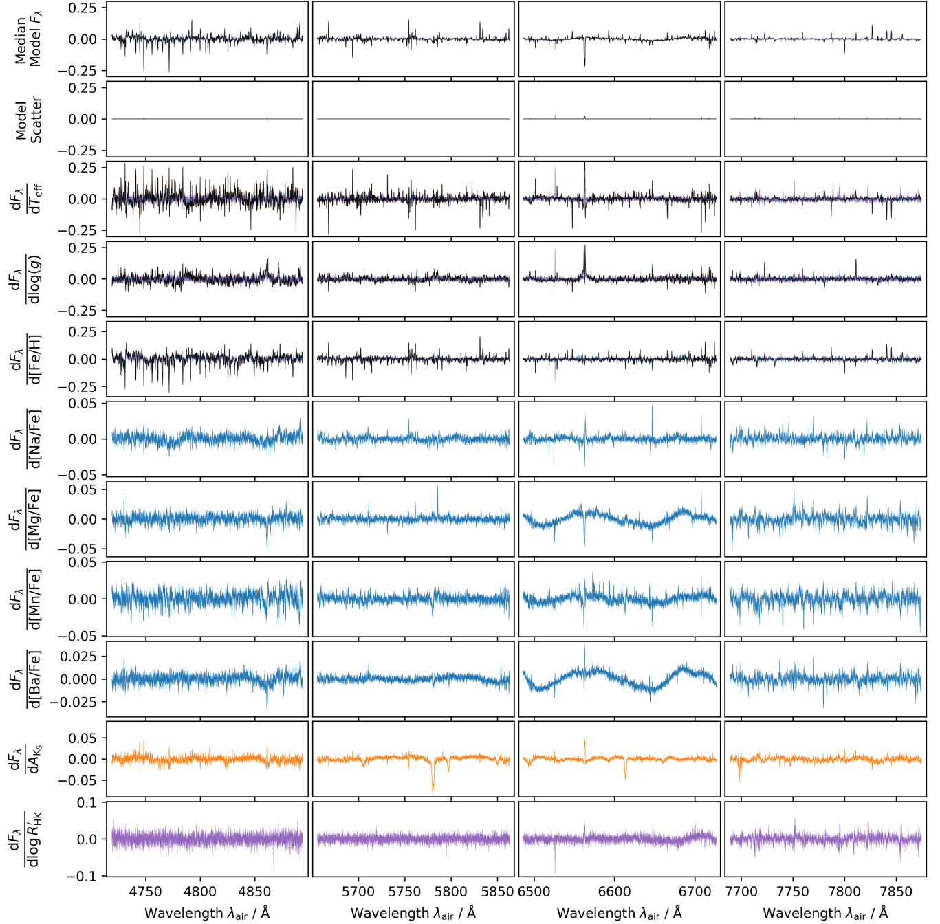
FIG. 8.— Selected coefficients across wavelength for Models M1, M2, M3, and M4. Lines show the median coefficient across the five cross-validation folds, and shaded regions show the full fold-to-fold range. Because the labels are internally centred and scaled, the coefficients describe the local residual response near the centre of each training-label distribution.
