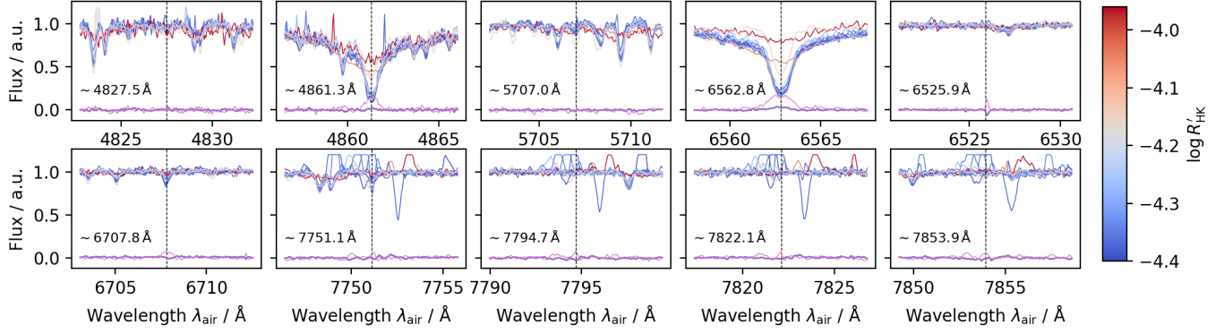
FIG. 10.— Observed flux for the 15 stars with highest \log R'_{\text{HK}} of the activity sample as well as linear and quadratic coefficients of \log R'_{\text{HK}} (thick and thin purple lines) for selected wavelength regions.
